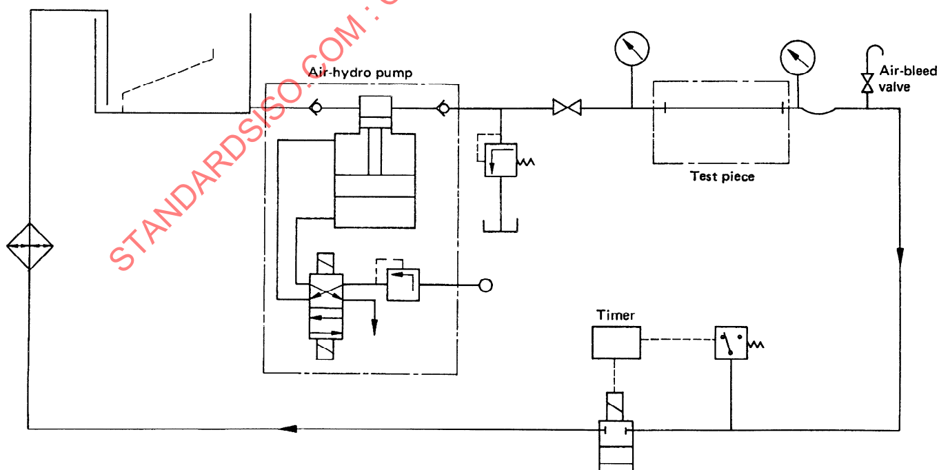
Figure A.2 — Suitable diagrammatic impulse test circuit
