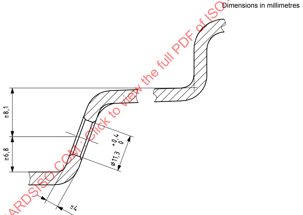
Figure 3 — Valve hole dimensions for snap-in valves
