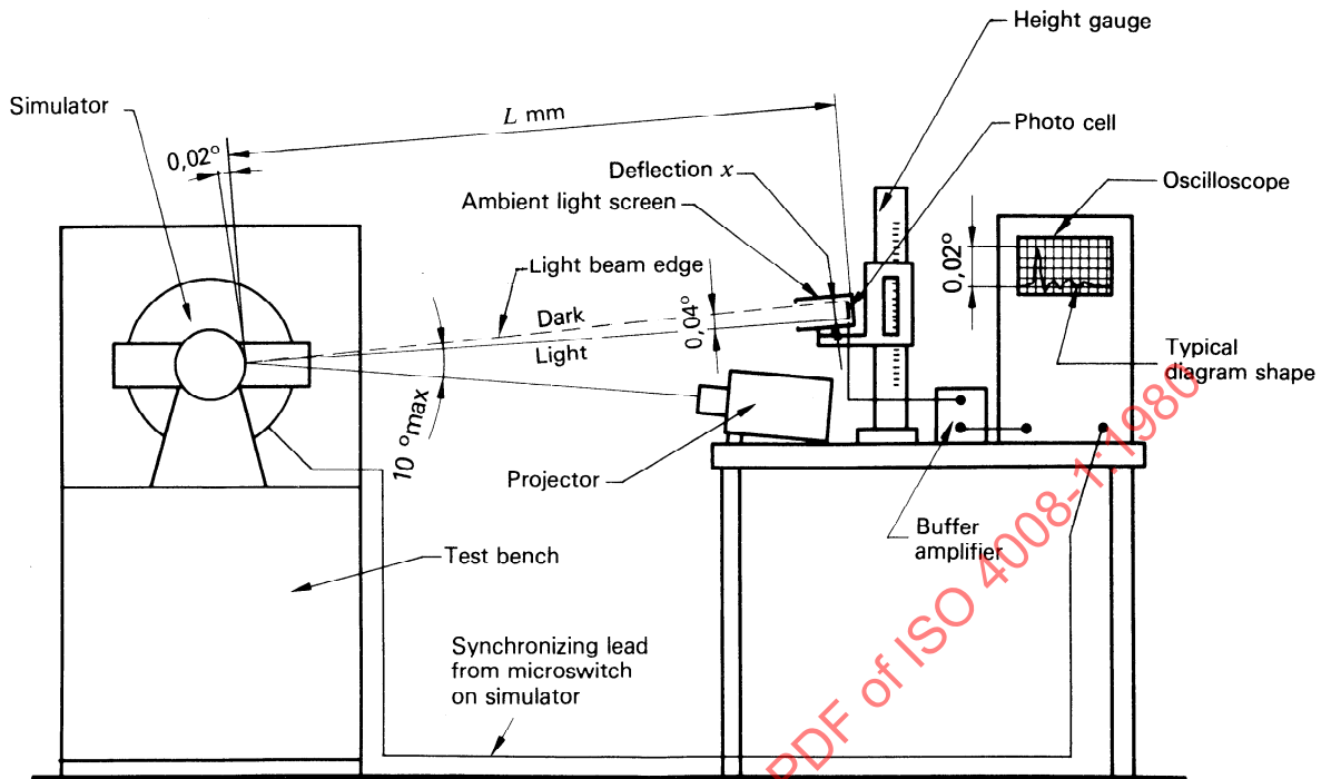
Figure 8 — Sketch of preferred apparatus in use
