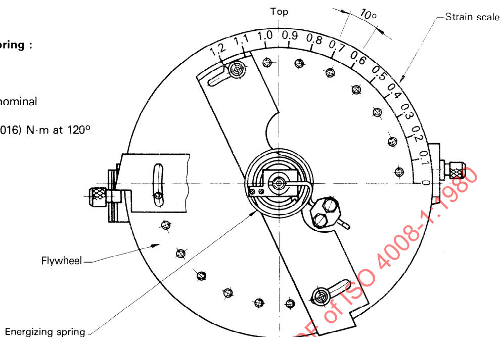
Figure 3 — Simulator, front elevation
