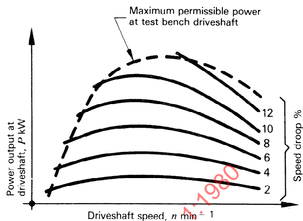
Figure 1 — Test bench power and speed droop characteristics — Graph 1
