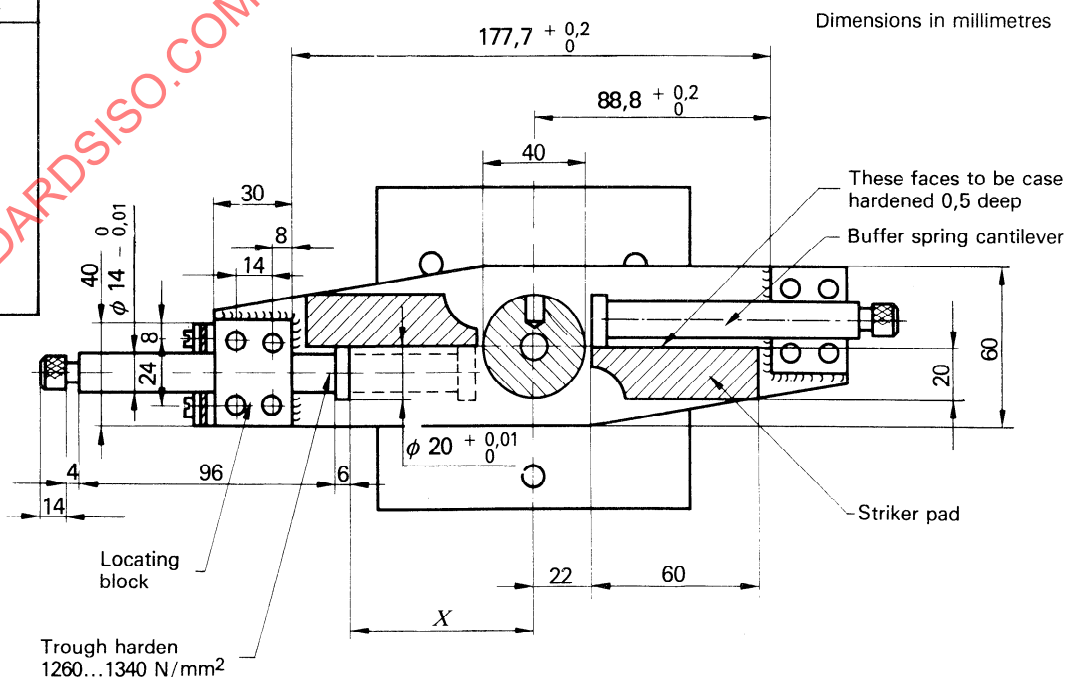
Figure 4 — Simulator, section B-B (see figure 6)
