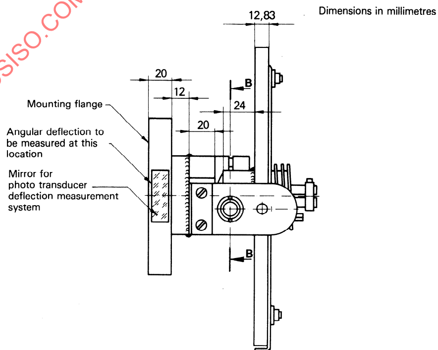
Figure 6 — Simulator, side elevation
