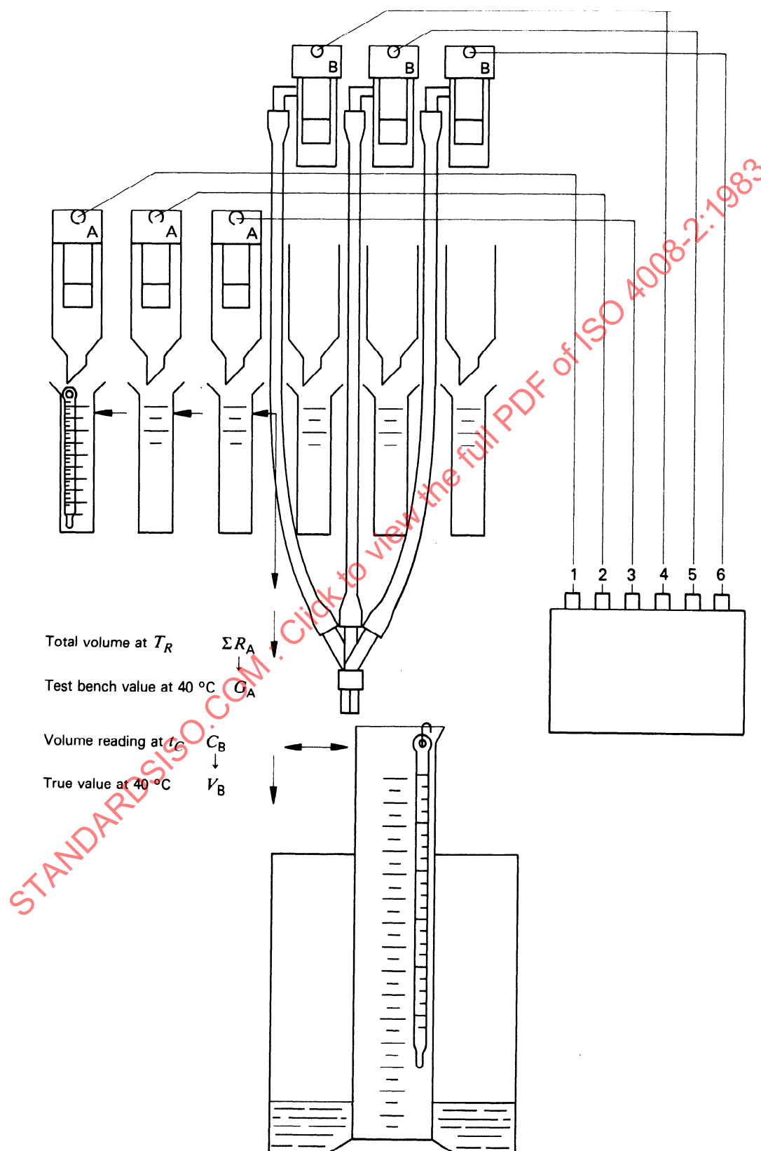
Figure 5 — Reversal of the measuring systems for stage 2
