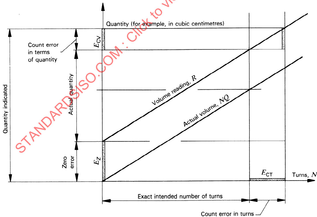
Figure 1 — Zero and count errors
