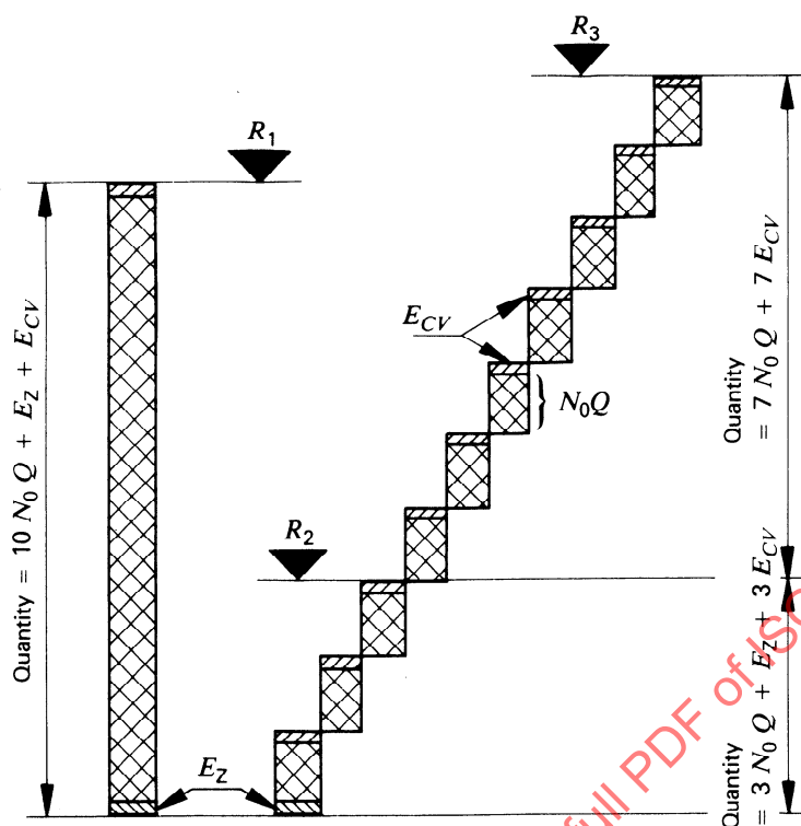
Figure 2 — Diagram showing the principle of the field test
