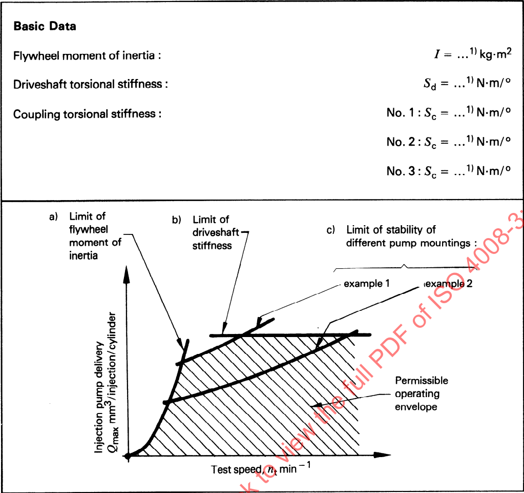
Figure 1 — Test bench permissible operating envelope and basic data (Reproduced from ISO 4008-1, figure 2)
