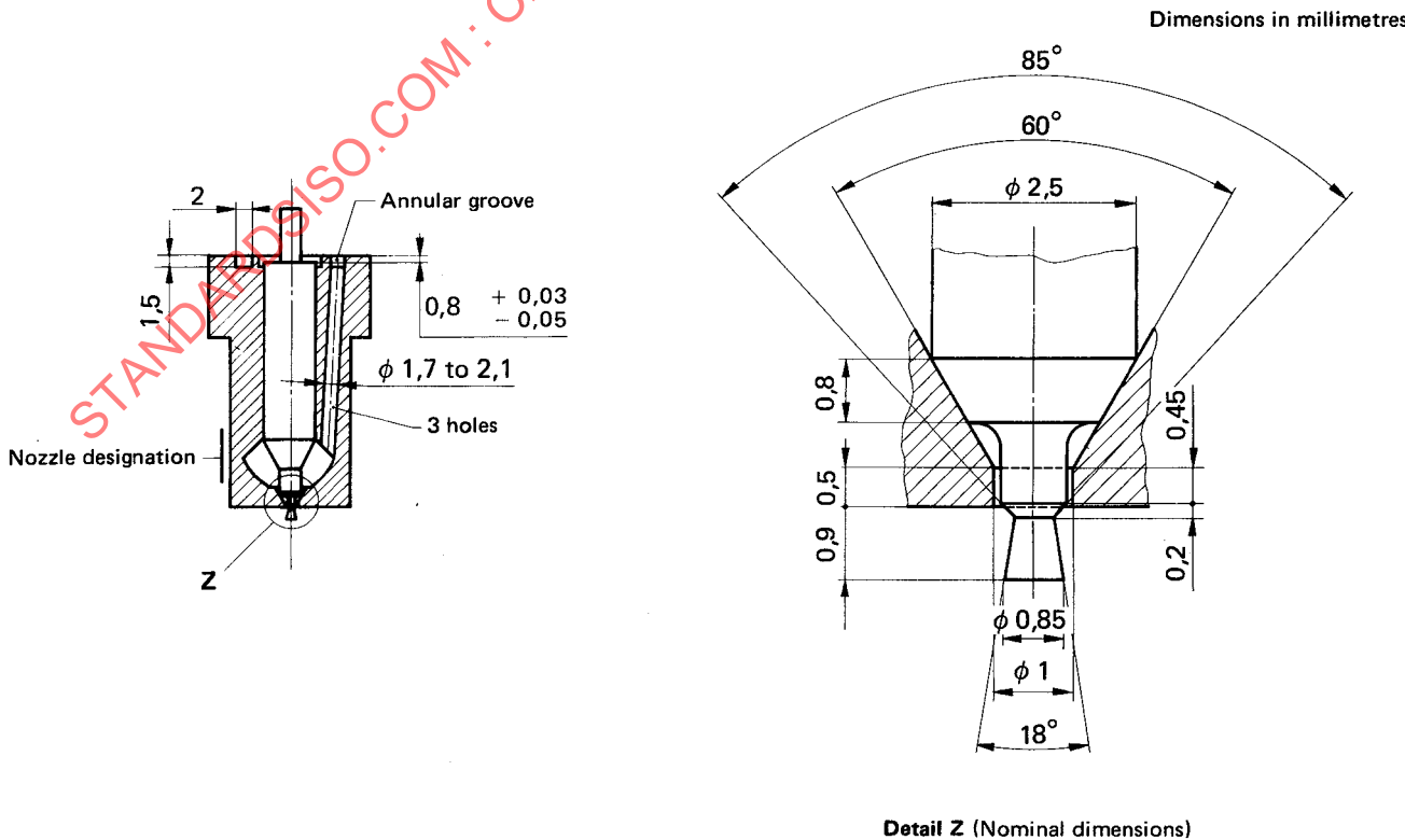
FIGURE 1 – Nozzle cross-section
