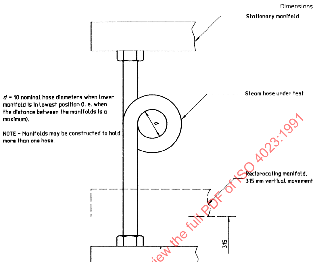
Figure 3 — Schematic diagram of arrangement for vertical flexing test (method C)
