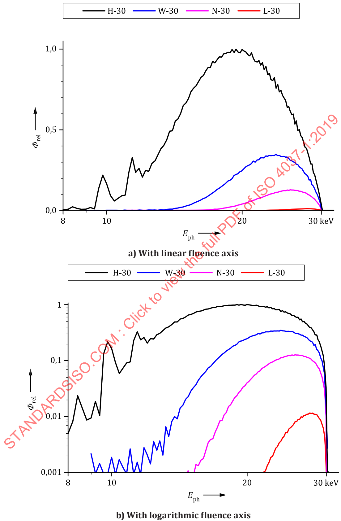
Figure 1 — Fluence spectra for a generating voltage of 30 kV with increasing filtration
