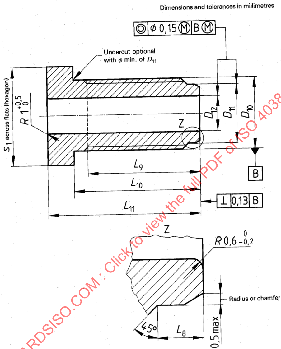
Figure 5 — Male fittings
