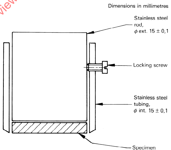
Figure 5 — Mould (7.9.1.1) for water sorption and solubility test (see 7.9)
