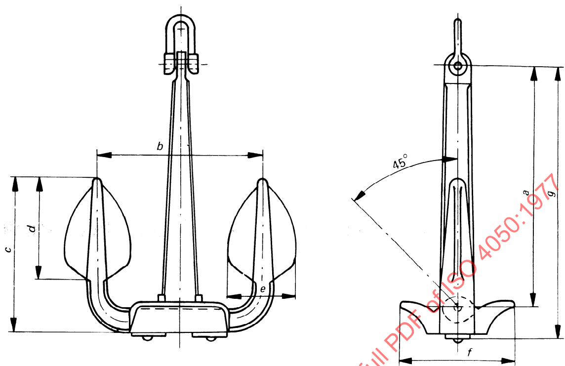
FIGURE 1 — “Rhine” stockless anchor
