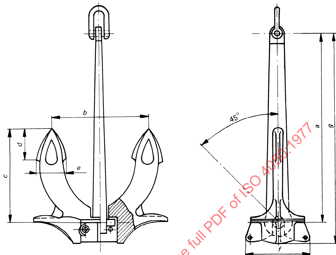
FIGURE 2 — Hall's stockless anchor
