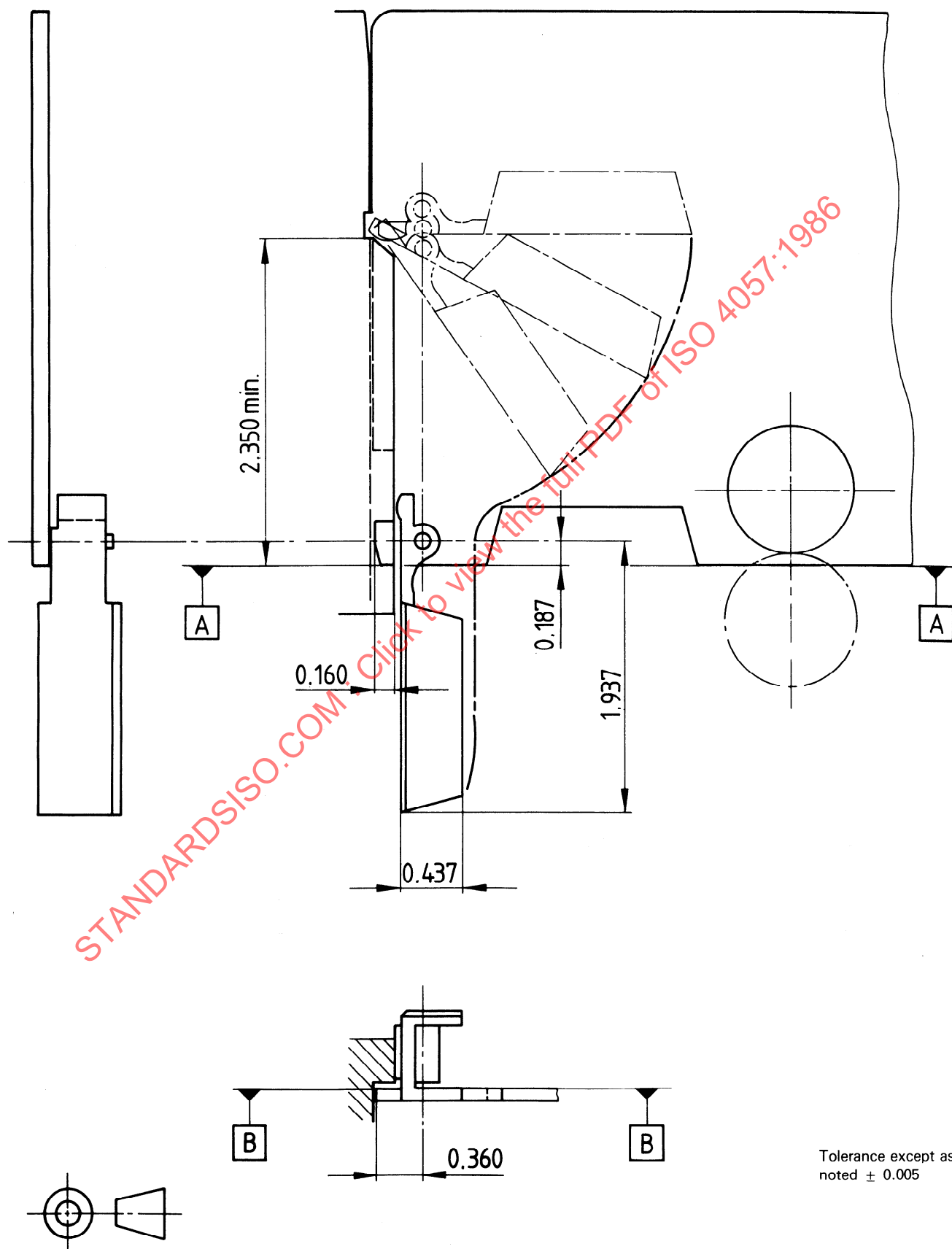
Figure 7b) — Cartridge door profile
