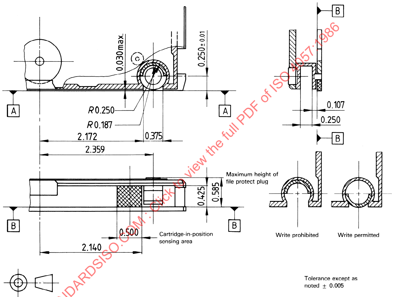
Figure 6b) — File protect and cartridge-in-position sensing
