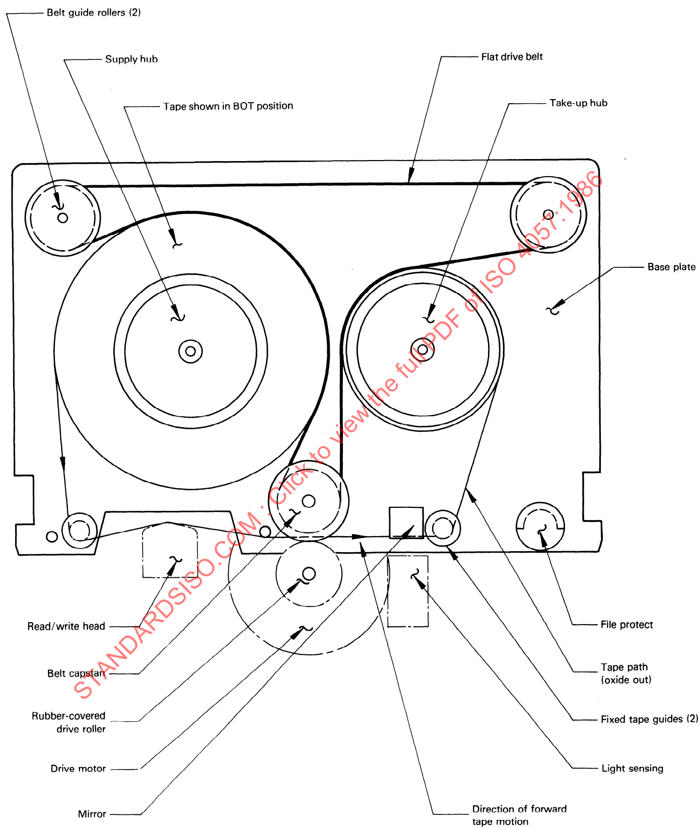
Figure 2 — Cartridge diagram
