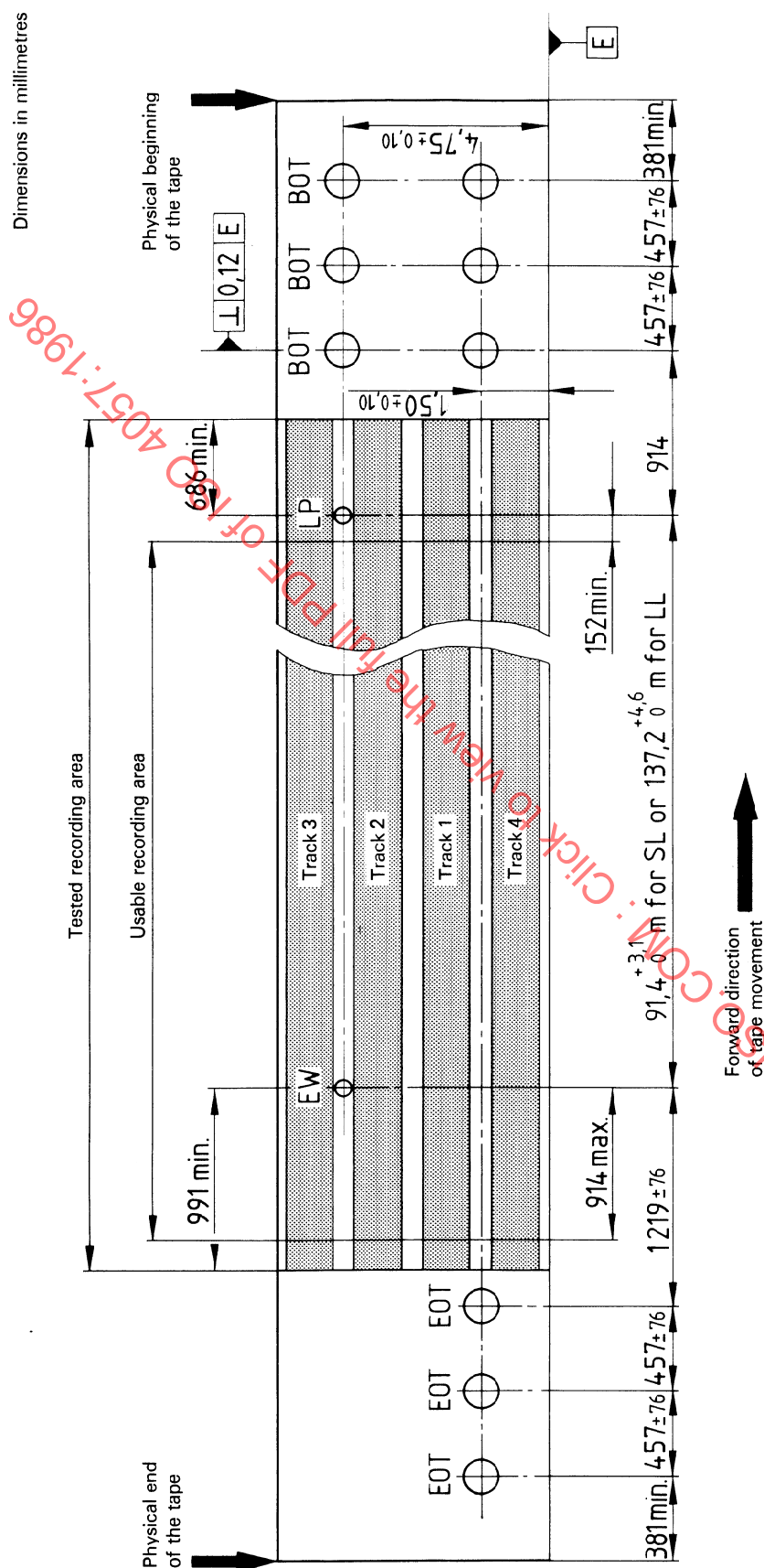
Figure 1a) — Position of the markers and recording areas (magnetic surface shown)
