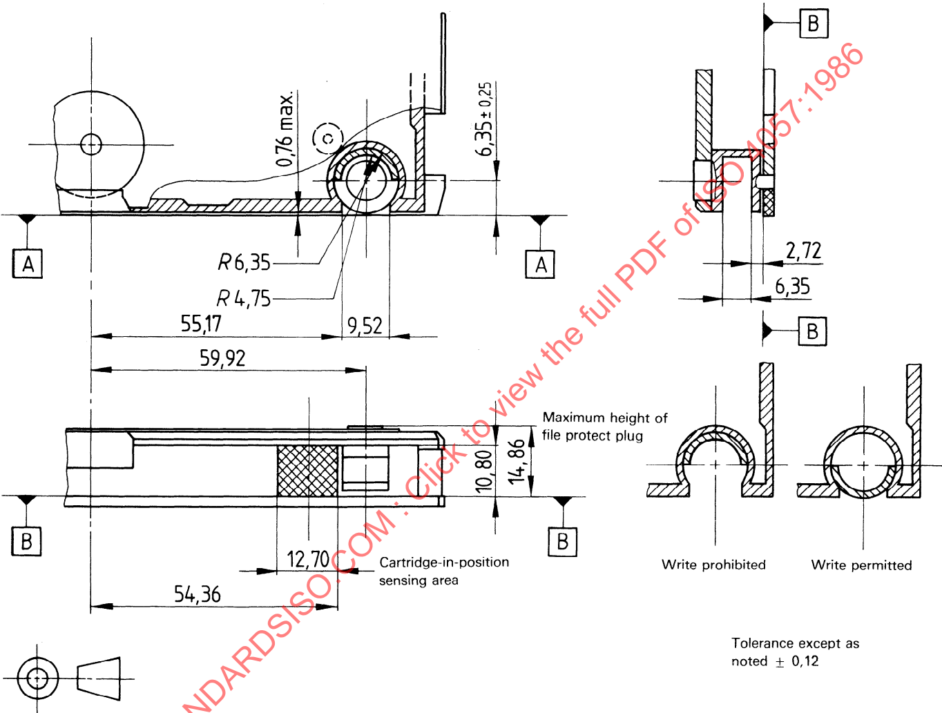
Figure 6a) — File protect and cartridge-in-position sensing
