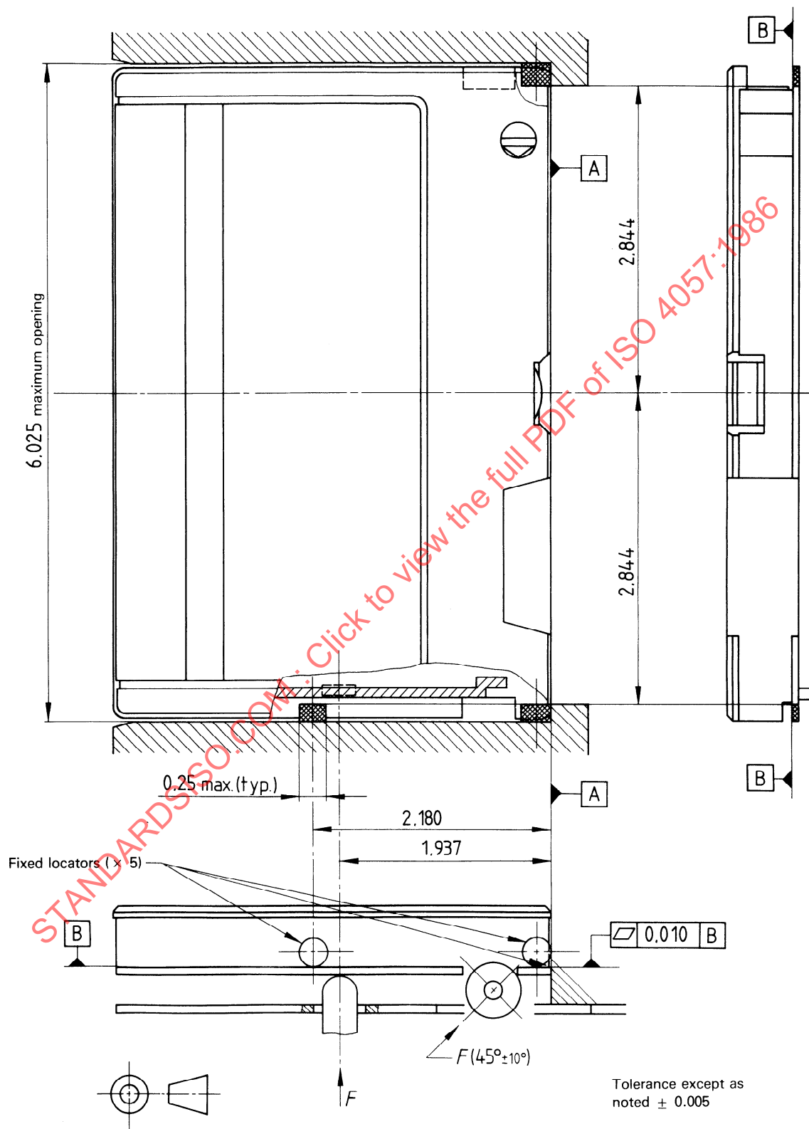
Figure 4b) — Cartridge locating planes
