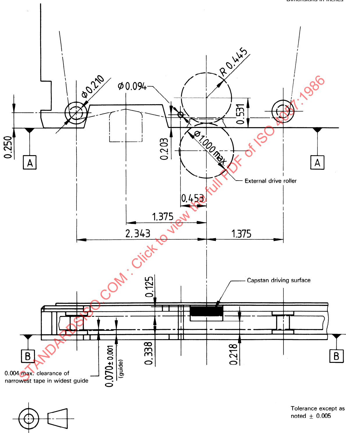
Figure 9b) — Tape path and drive dimensions
