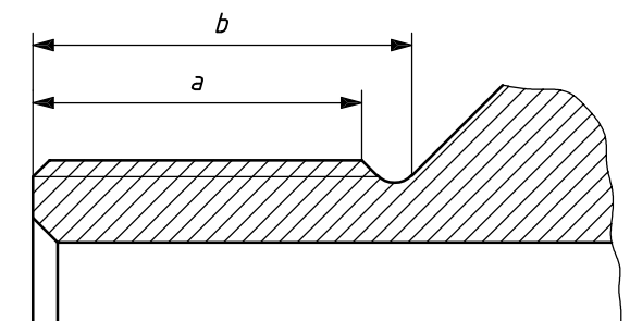
Figure 2 — Threaded connection
