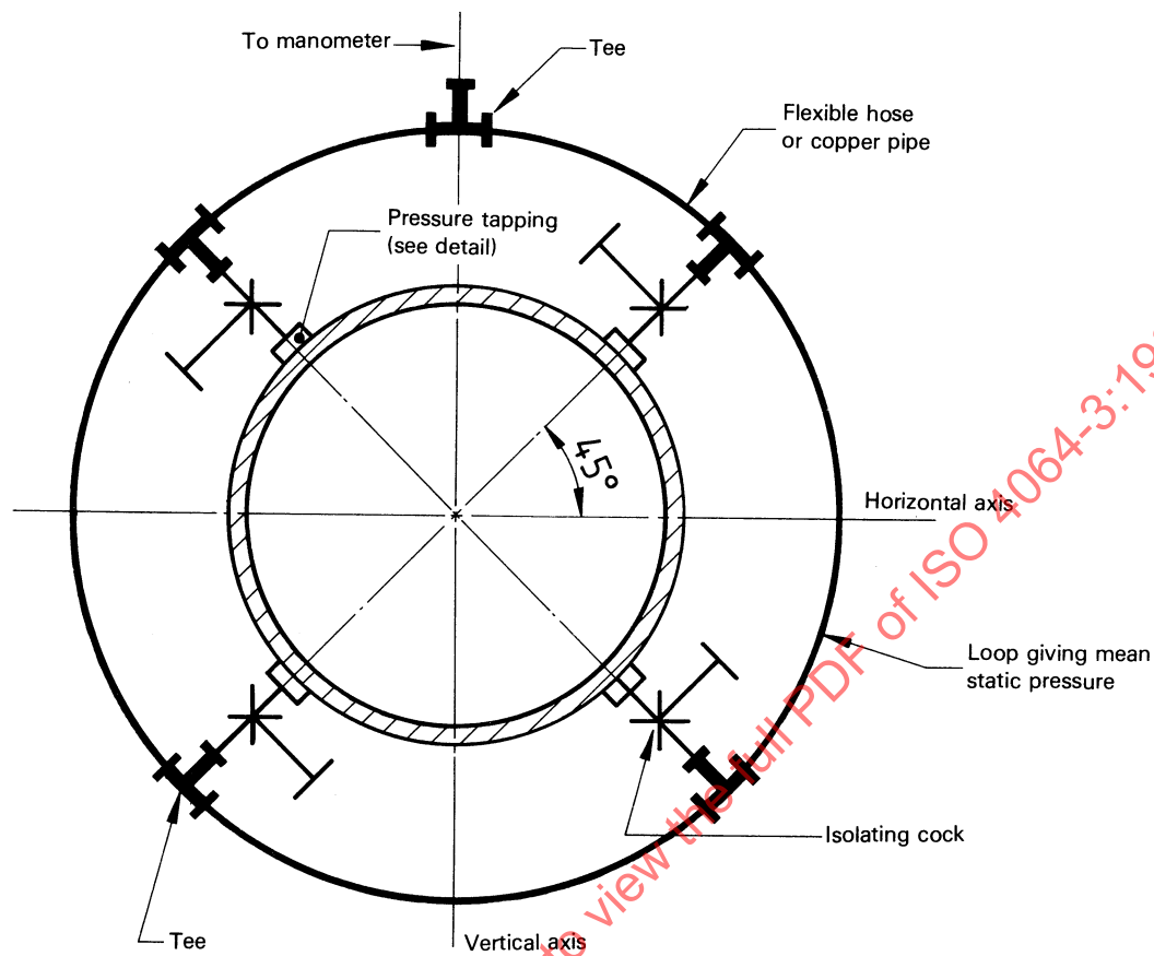
Cross-section through pipe and pressure tapings
