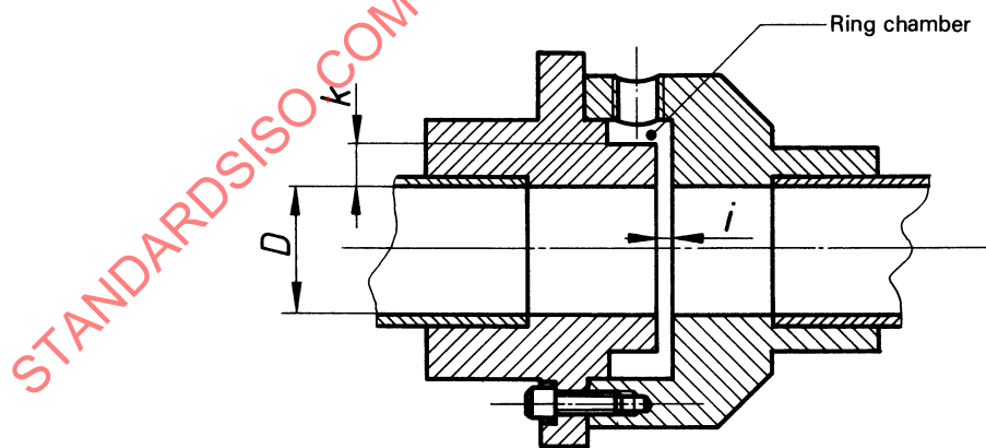
Figure 3 — Example of slit type of pressure tapping with ring chamber, suitable for small/medium diameter test sections
