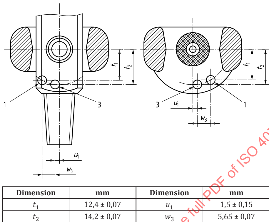
Figure 12 — Outlet connection for ethylene
