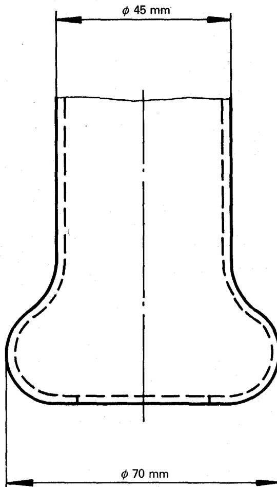
Figure — Suitable mount
