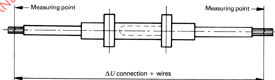
Figure 5 — Voltage drop test measuring points
