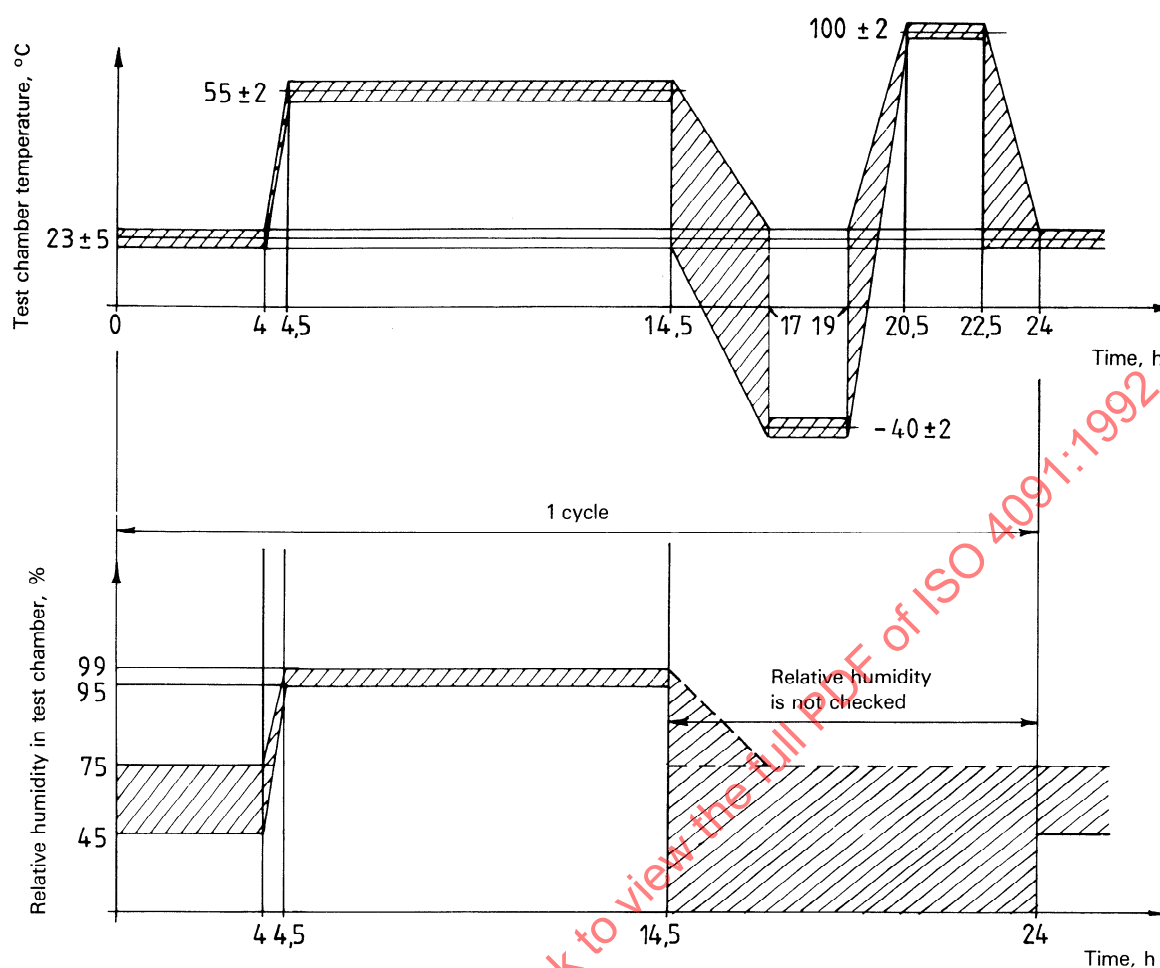
Figure 4 — Temperature/humidity test
