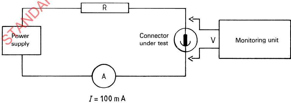
Figure 2 — Resistance monitor
