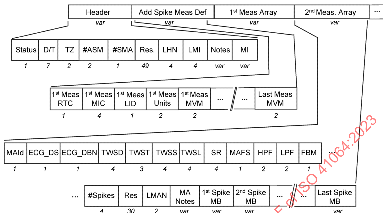
Figure 24 — Overview of the data part of Section 17
