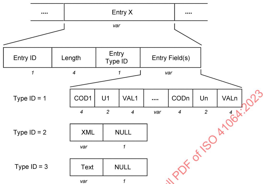
Figure 26 — Overview of the data content of a single annotation Entry
