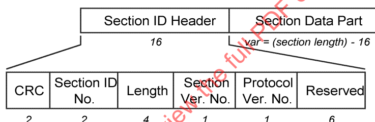
Figure 2 — Section layout overview
