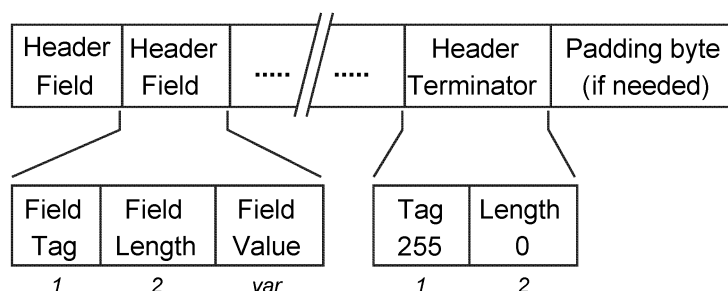
Figure 4 — Overview of the “Header information” section data part
