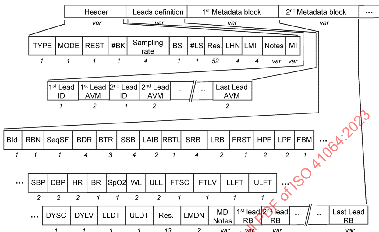
Figure 17 — Overview of the data part of Section 13
