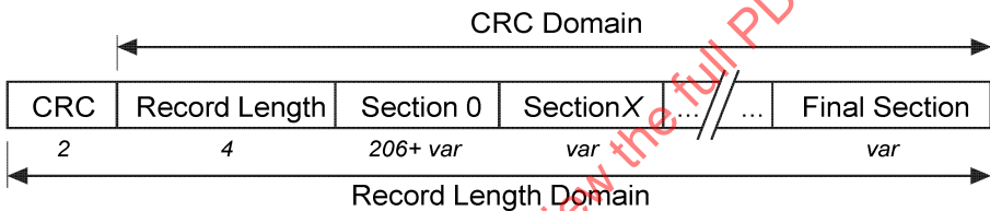
Figure 1 — SCP-ECG record overview
