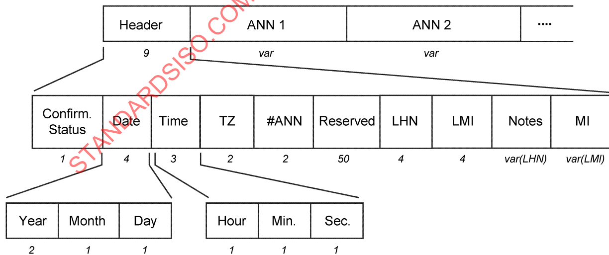
Figure 27 — Overview of the data part of Section 18
