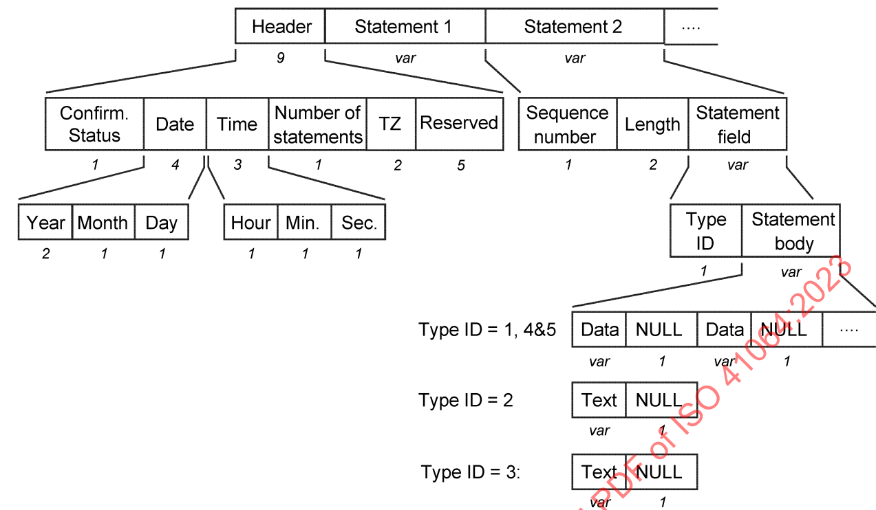
Figure 15 — Overview of the data part of Section 11
