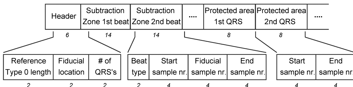
Figure 7 — Overview of the data part of section 4
