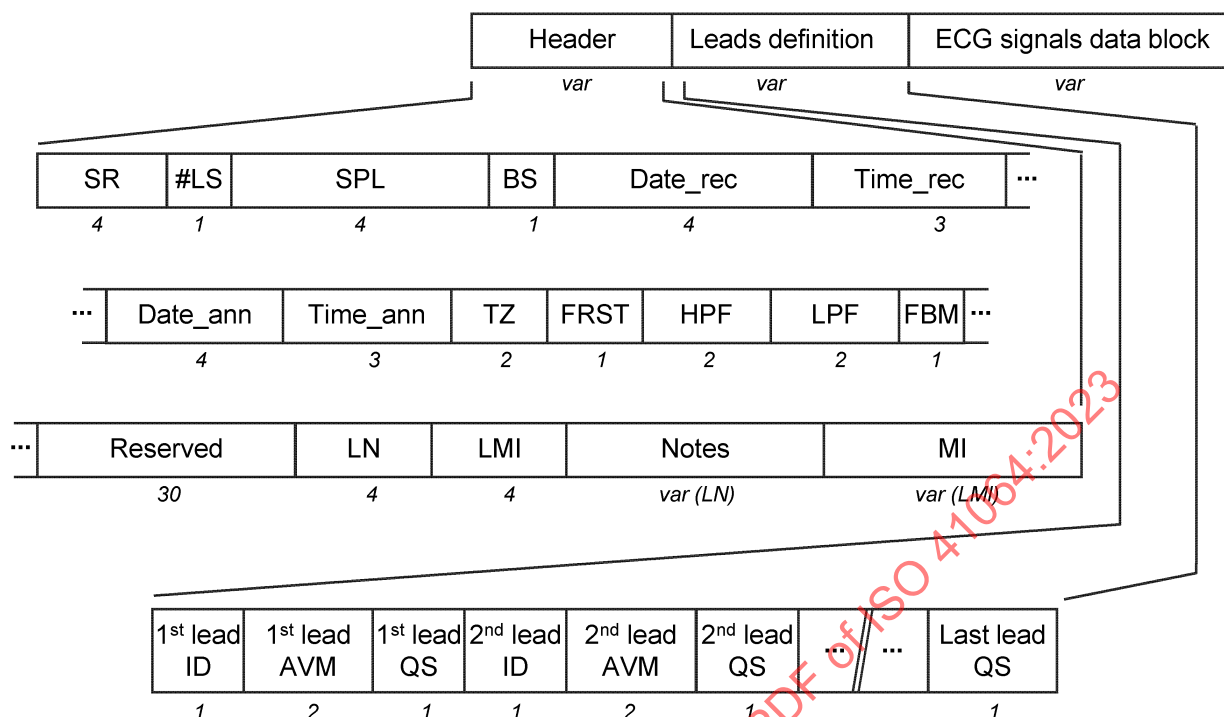
Figure 16 — Overview of the data part of Section 12
