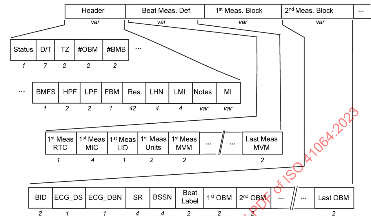
Figure 22 — Overview of the data part of Section 16
