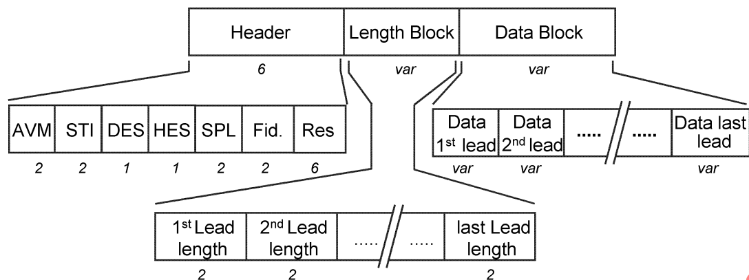
Figure 8 — Overview of the data part of the encoded type 0 reference beat section
