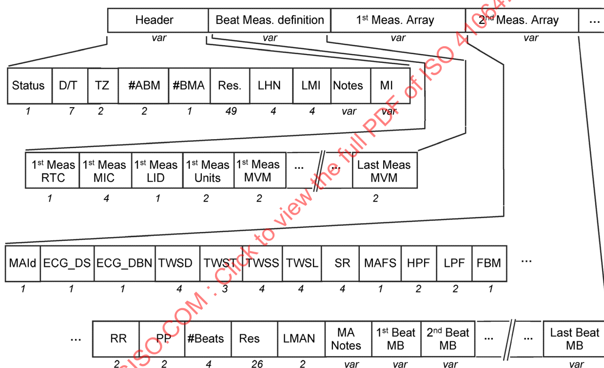
Figure 20 — Overview of the data part of Section 15
