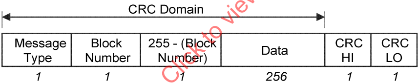
Figure C.2 — CRC-CCITT error detection
