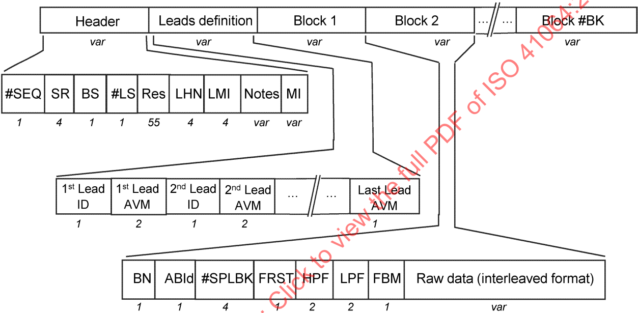
Figure 18 — Overview of the data part of Section 14
