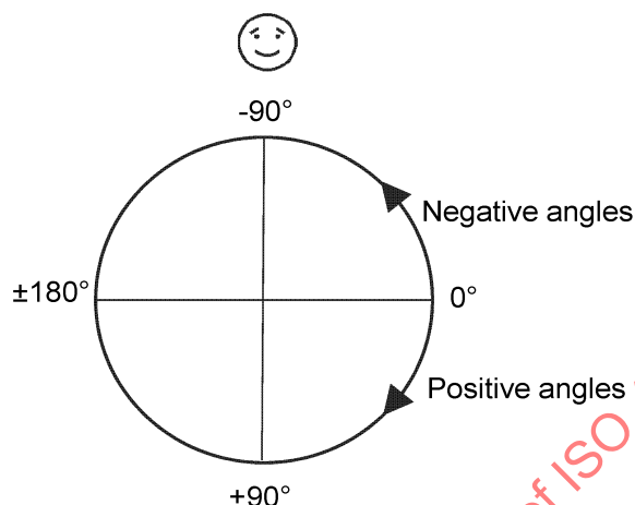
Figure 10 — Angle definition for the electrical axes in the frontal plane
