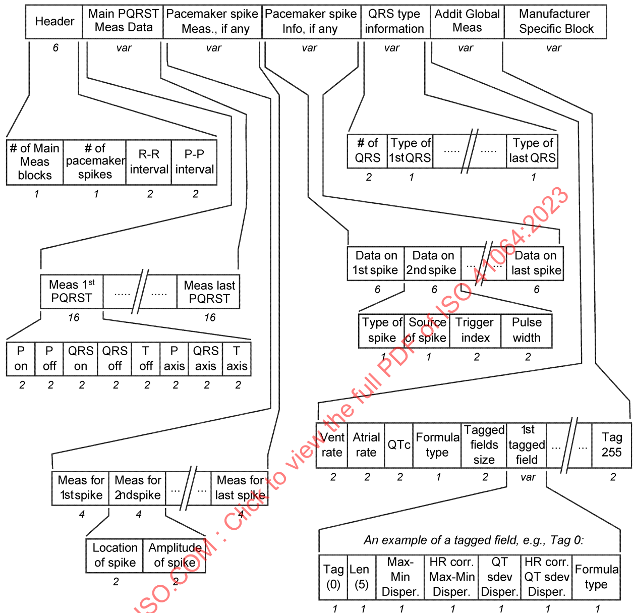
Figure 12 — Overview of the data part of the global measurements section
