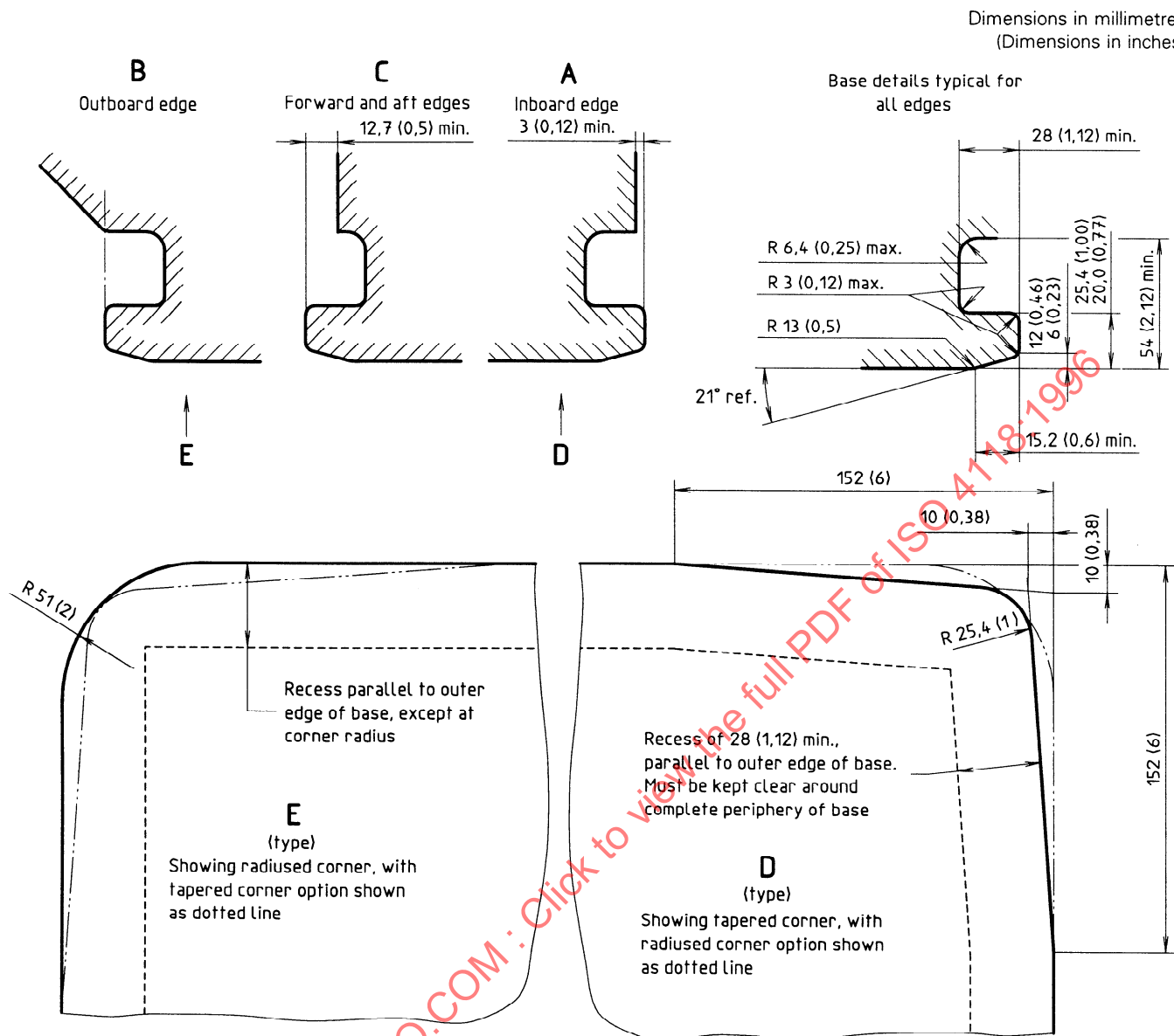
Figure 1 — Details of the container base — Option A
