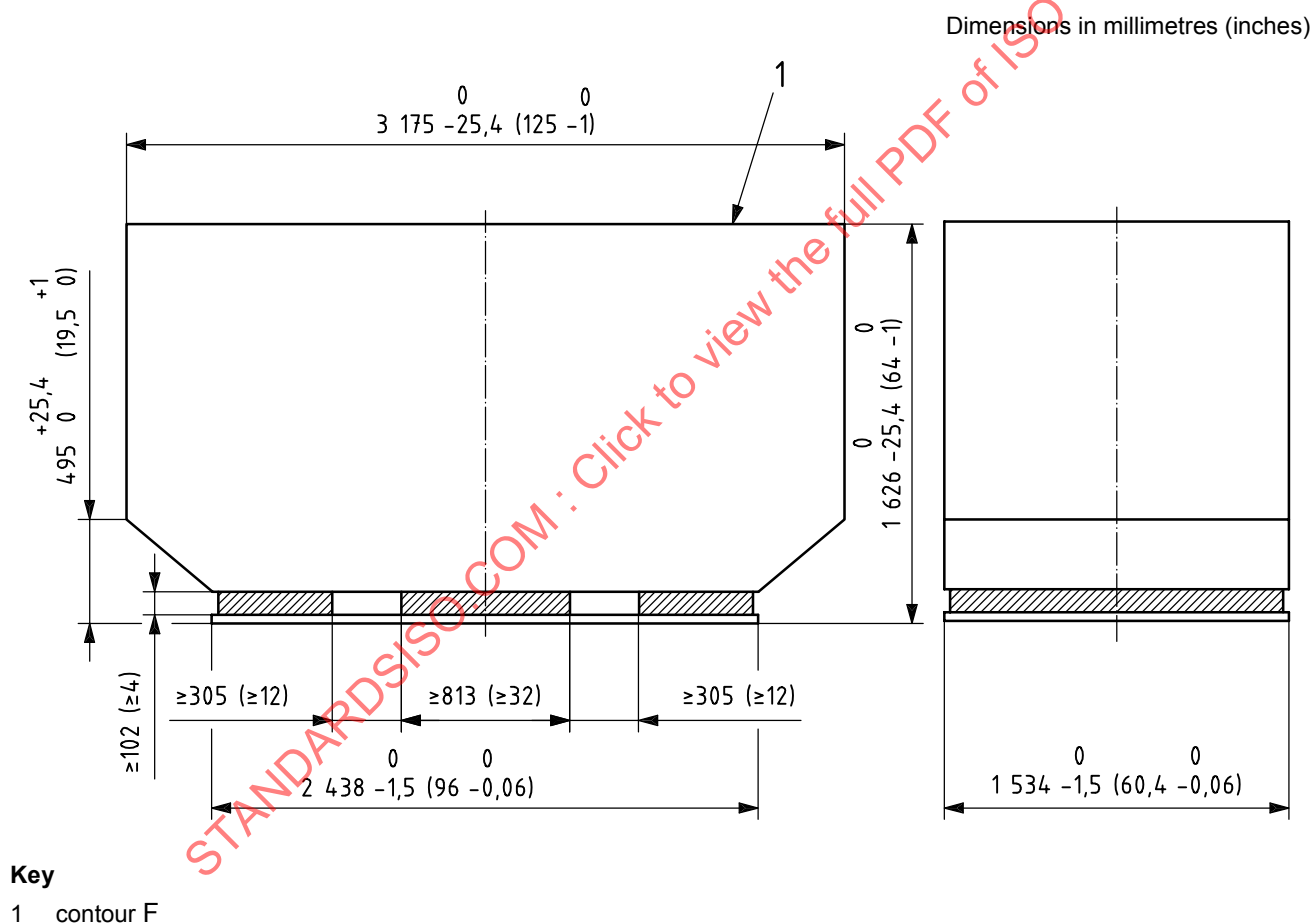
Figure G.1 — Dimensions of code DQF full-width contoured containers
