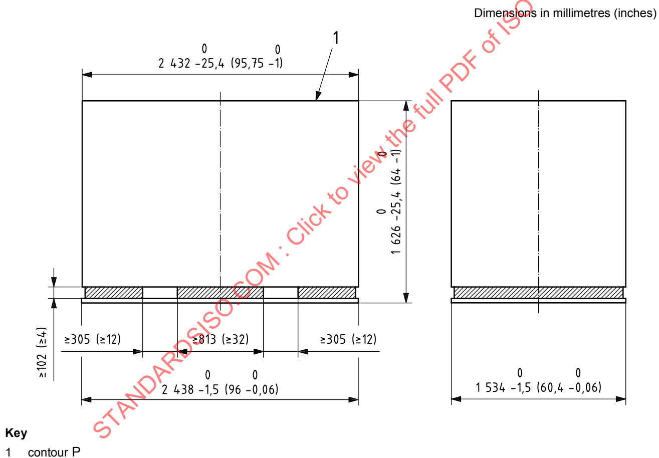
Figure H.1 — Dimensions of code DQP full-width rectangular containers
