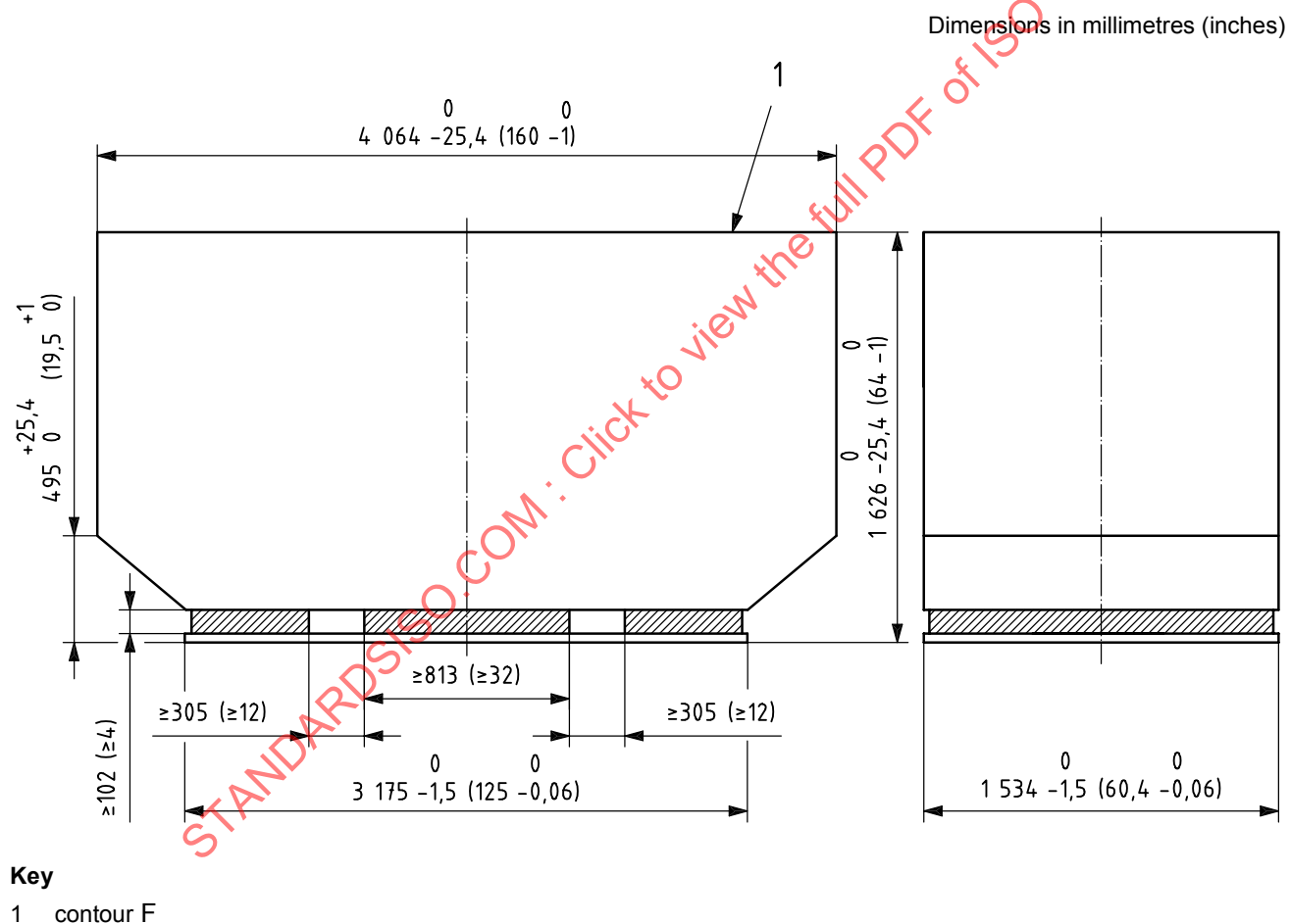
Figure D.1 — Dimensions of code DLF full-width contoured containers
