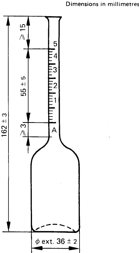
FIGURE 2 – Flask for sulphuric polymerization test (The flask is graduated at 20 °C)
