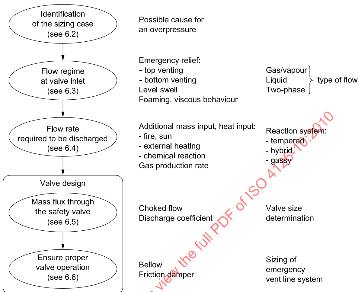
Figure 3 — Procedure of valve sizing
