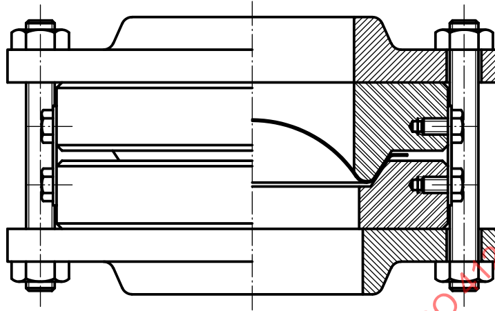
Figure 5 — Typical insert/capsule bursting disc holder
