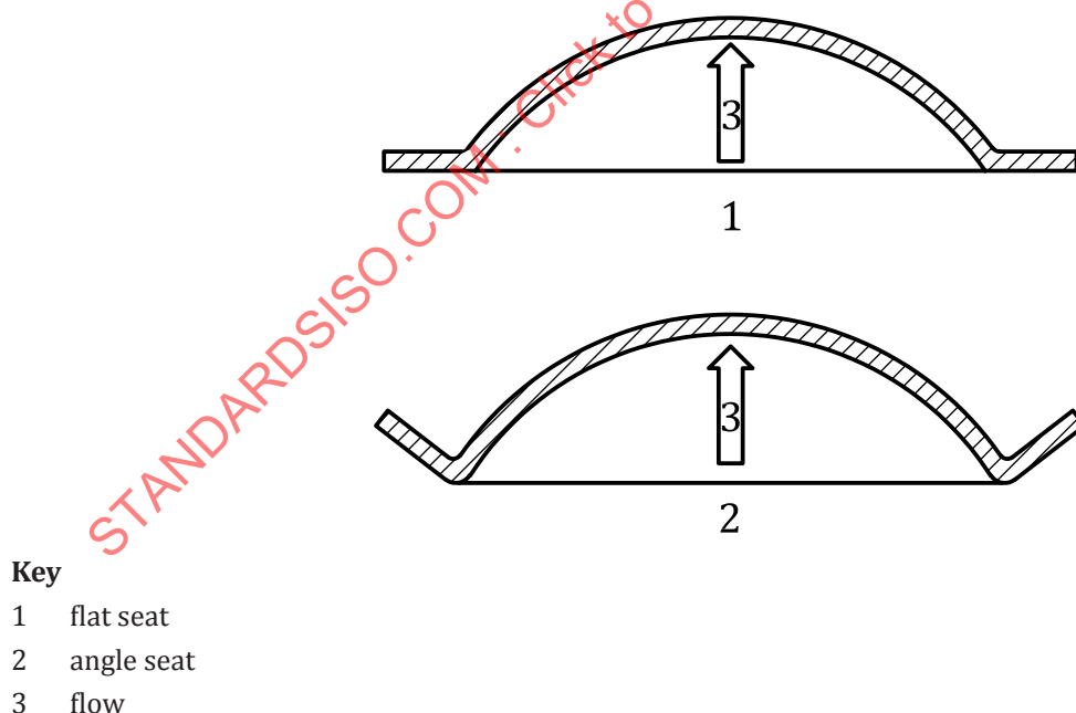
Figure 1 — Conventional domed bursting disc (Forward acting)
