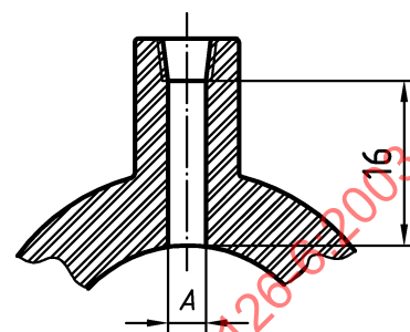
Figure E.1b – Pressure tap detail
