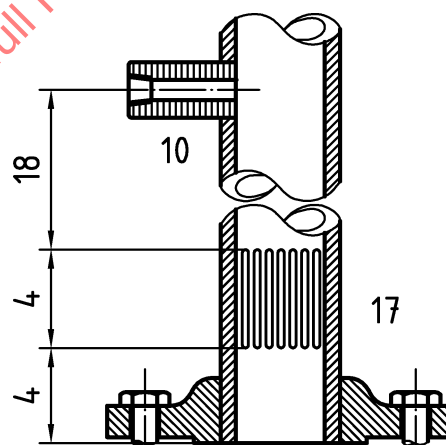
Figure E.1c – Remainder of test rig to be configured as the test rig without straightening vanes
