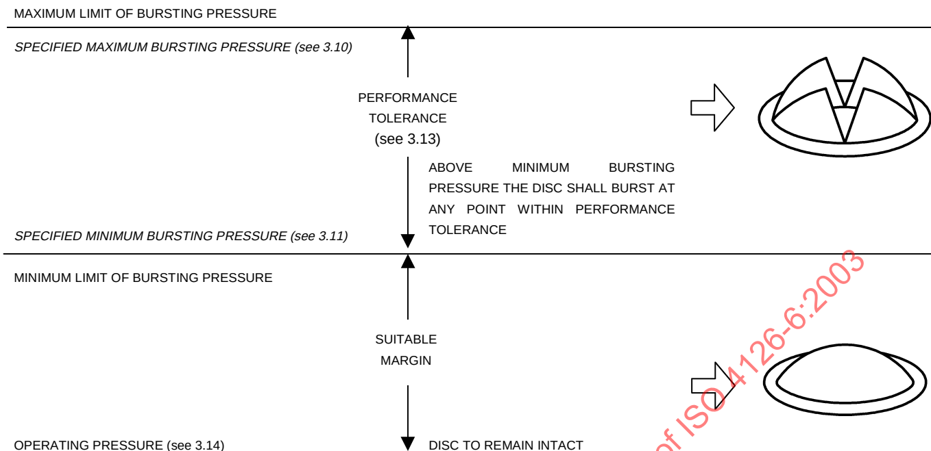
Figure 1a — Specified maximum bursting pressure and specified minimum bursting pressure with a coincident temperature
