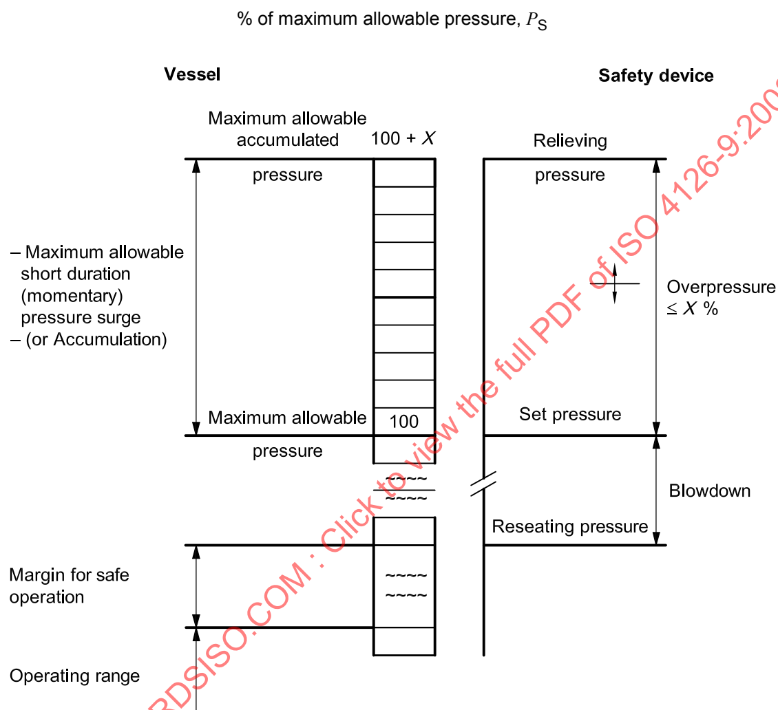
Figure A.1 — Safety valve applications — Safety valve certified at X\% overpressure or less
