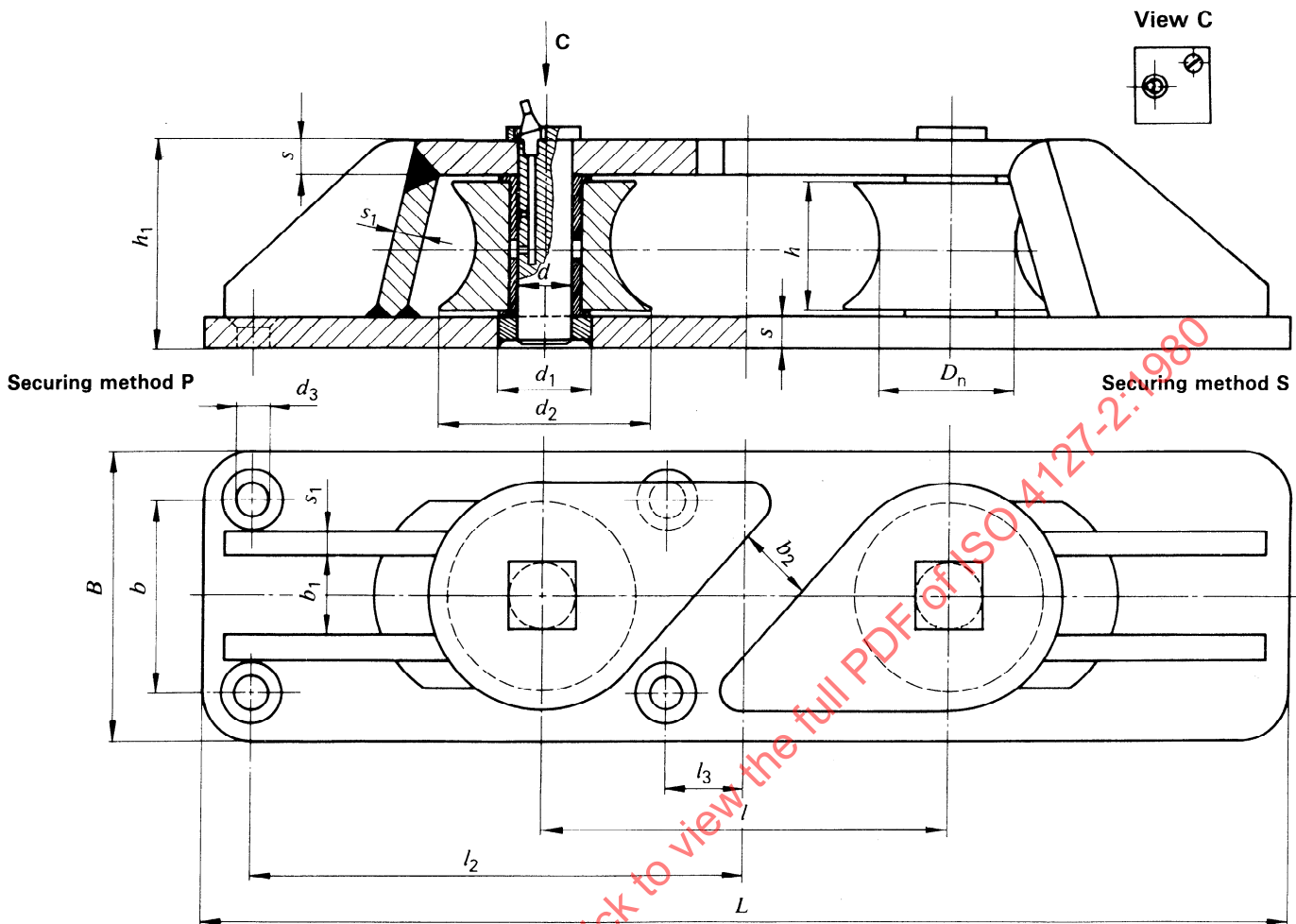
Figure 1 — Common roller fairlead (Type Z)
