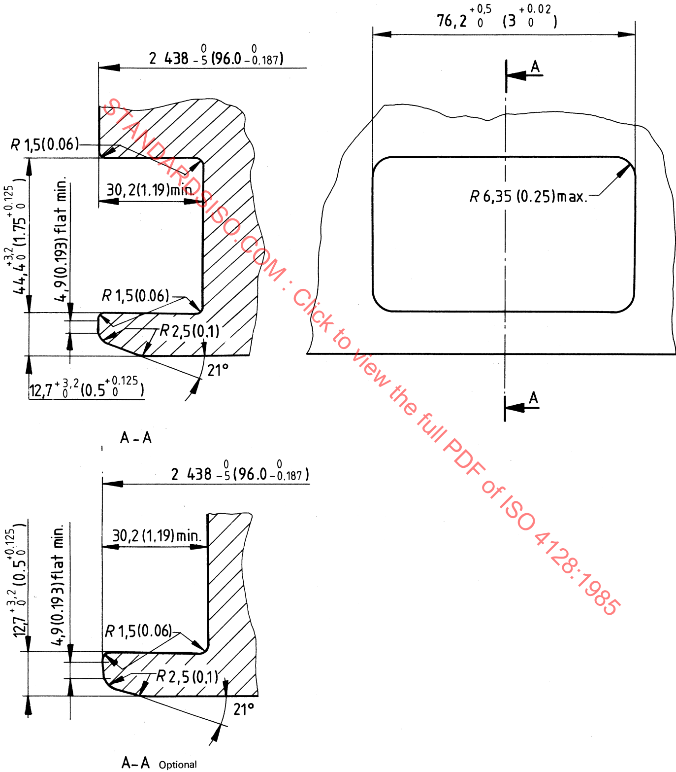
Figure 5 — Side slot detail
