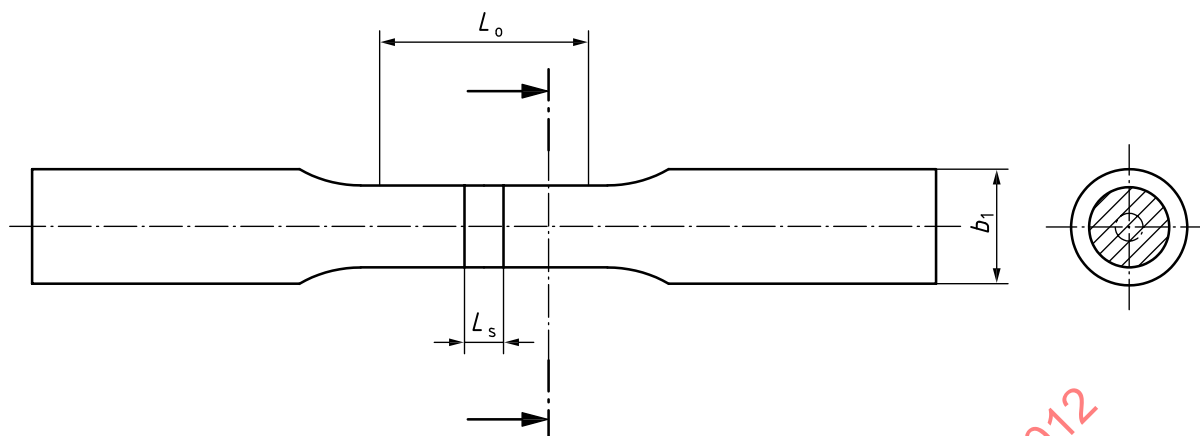
Figure 4 — Cylindrical test specimen for solid section
