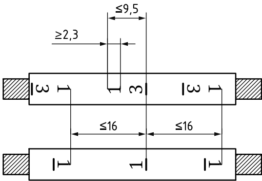
Figure 3 — Marking of cores
