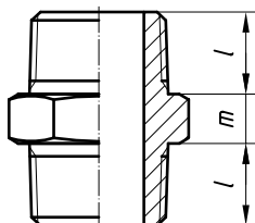
Figure 10 — Hexagon nipple N1
