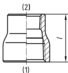
Figure 8 — Reducing socket S3
