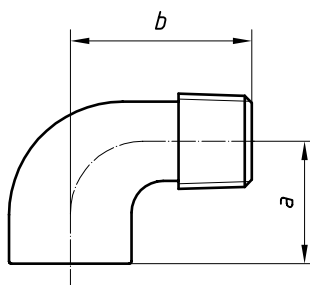
Figure 5 — Male and female elbow E4
