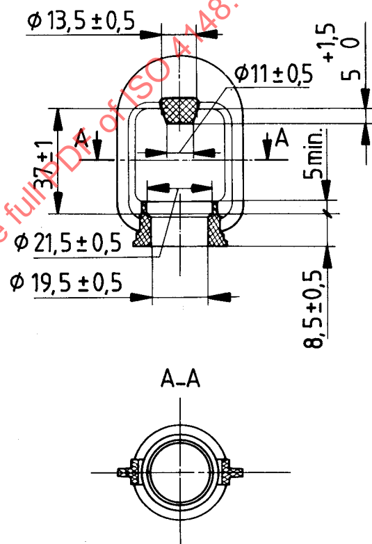
Figure 3 — Rubber cover for use when the special warning lamp (category A) is not mounted
