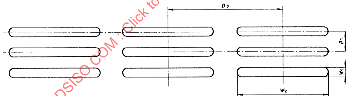
Figure B.1 — Slotted apertures — Arrangement in rows
