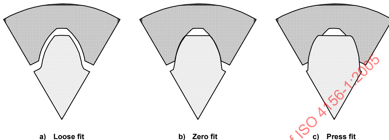
Figure 16 — Types of fit
