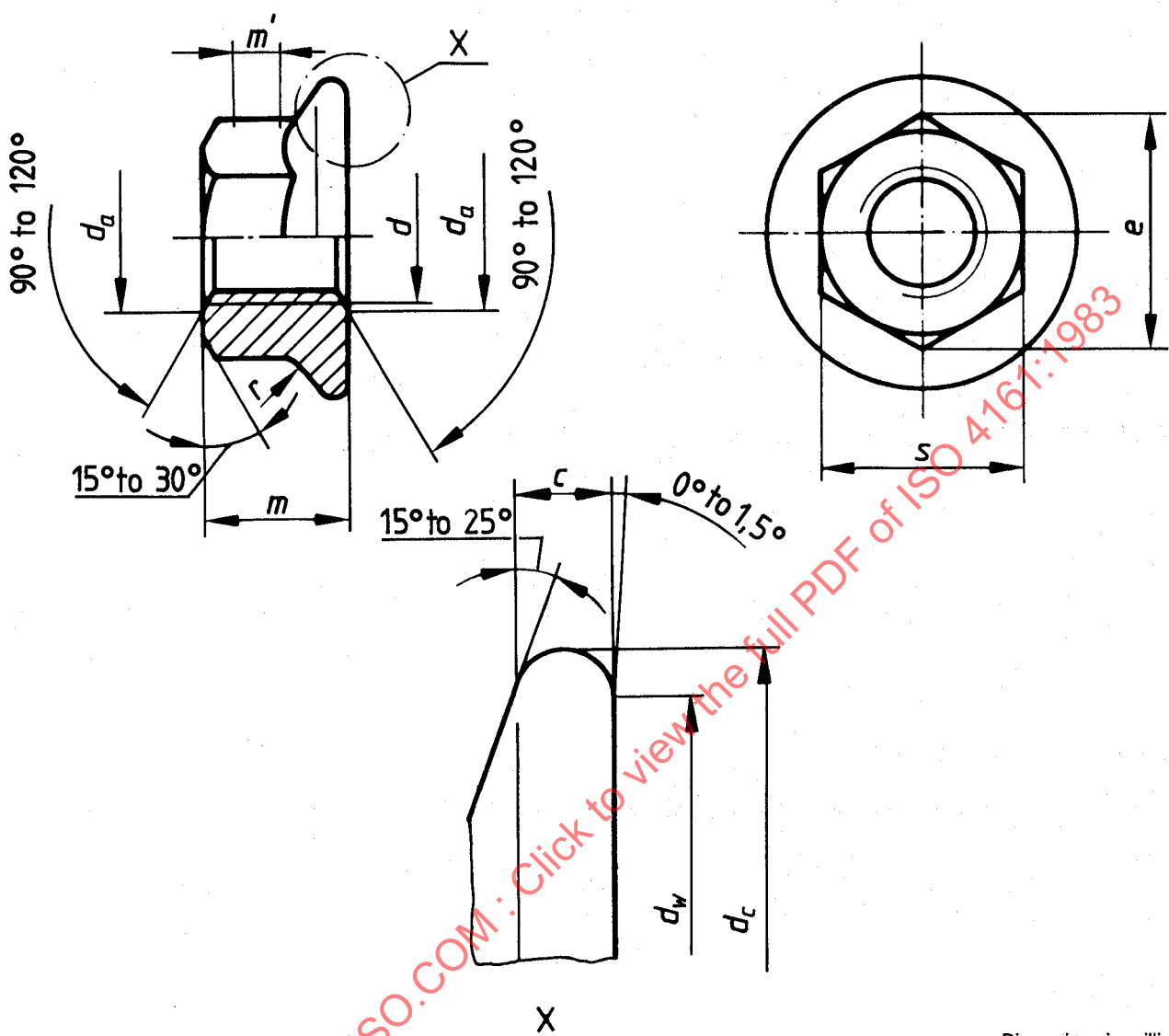
Dimensions in millimetres
