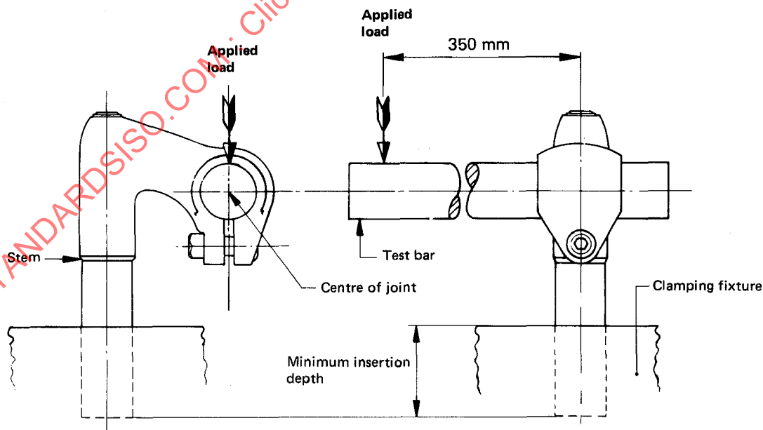
FIGURE 5 — Torque test on handlebar stem
