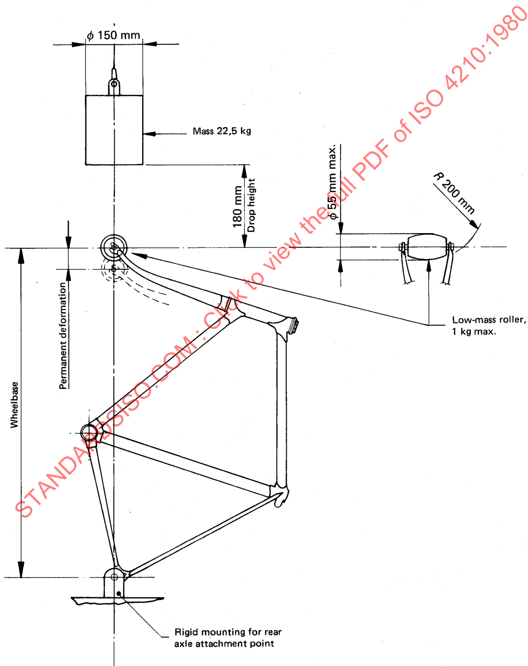
FIGURE 9 — Impact test (falling mass)
