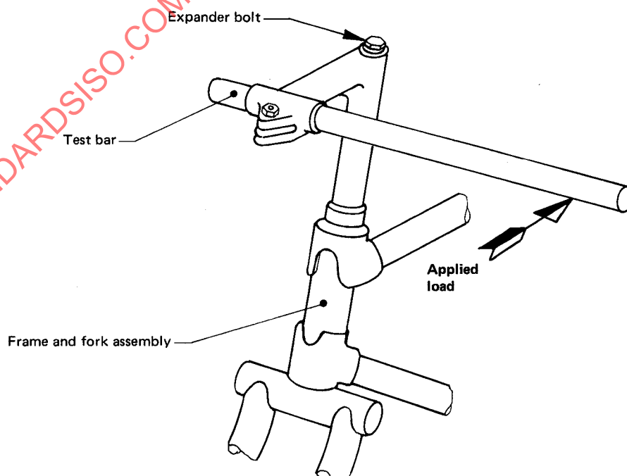
FIGURE 8 — Torque test on handlebar/fork clamping device
