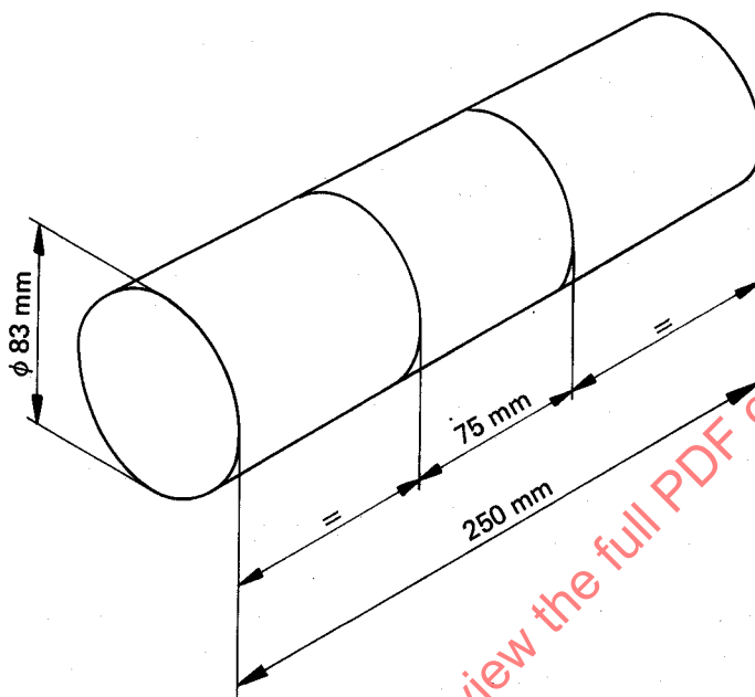
FIGURE 1 — Exposed protrusion test cylinder
