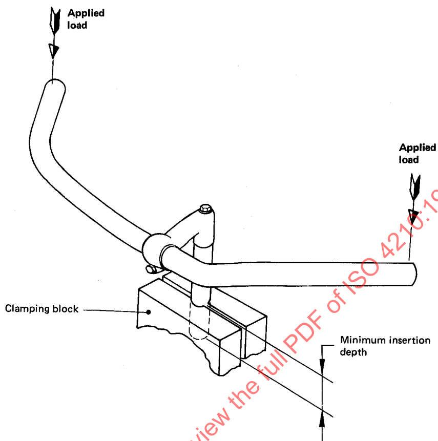
FIGURE 7 — Torque test on handlebar/stem assembly
