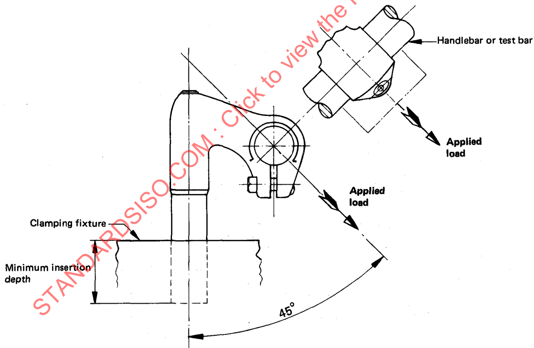
Figure 12 — Static load test on handlebar stem
