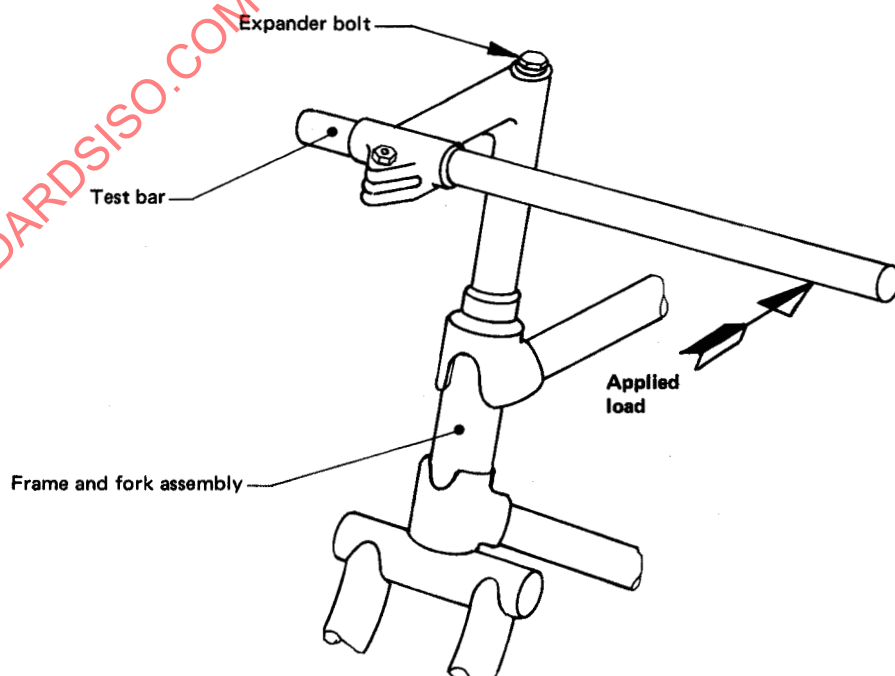
Figure 14 — Torque test on handlebar/fork clamping device
