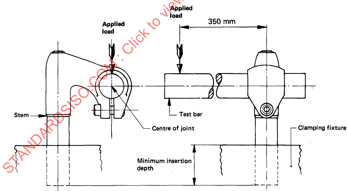
Figure 11 — Torque test on handlebar stem
