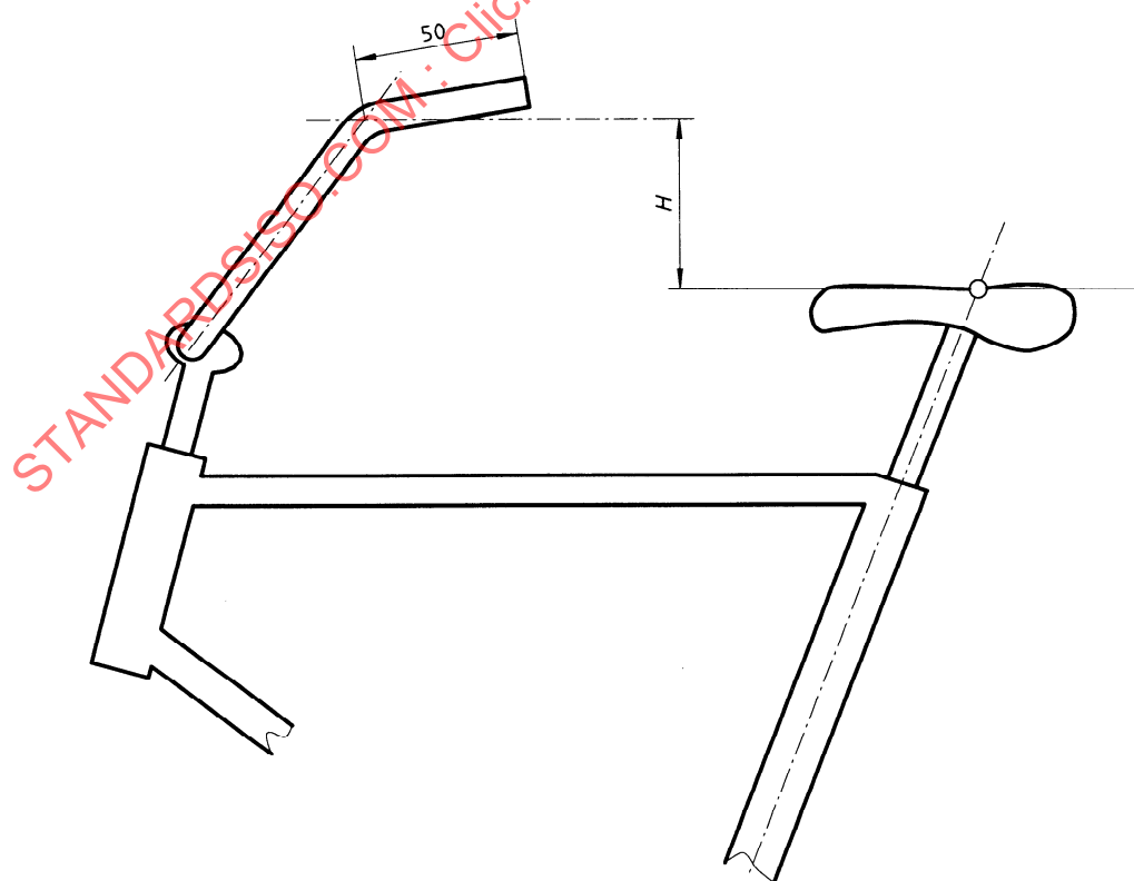
Figure 21 — High-rise handlebar; dimension H
