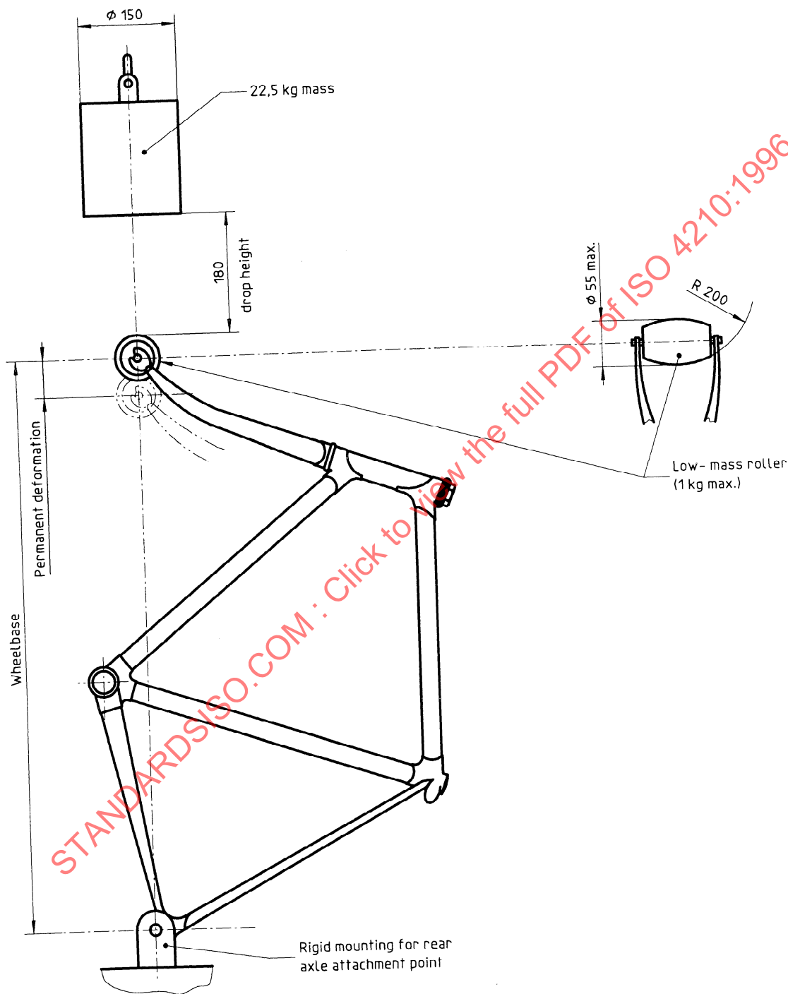
Figure 23 — Impact test (falling mass)
