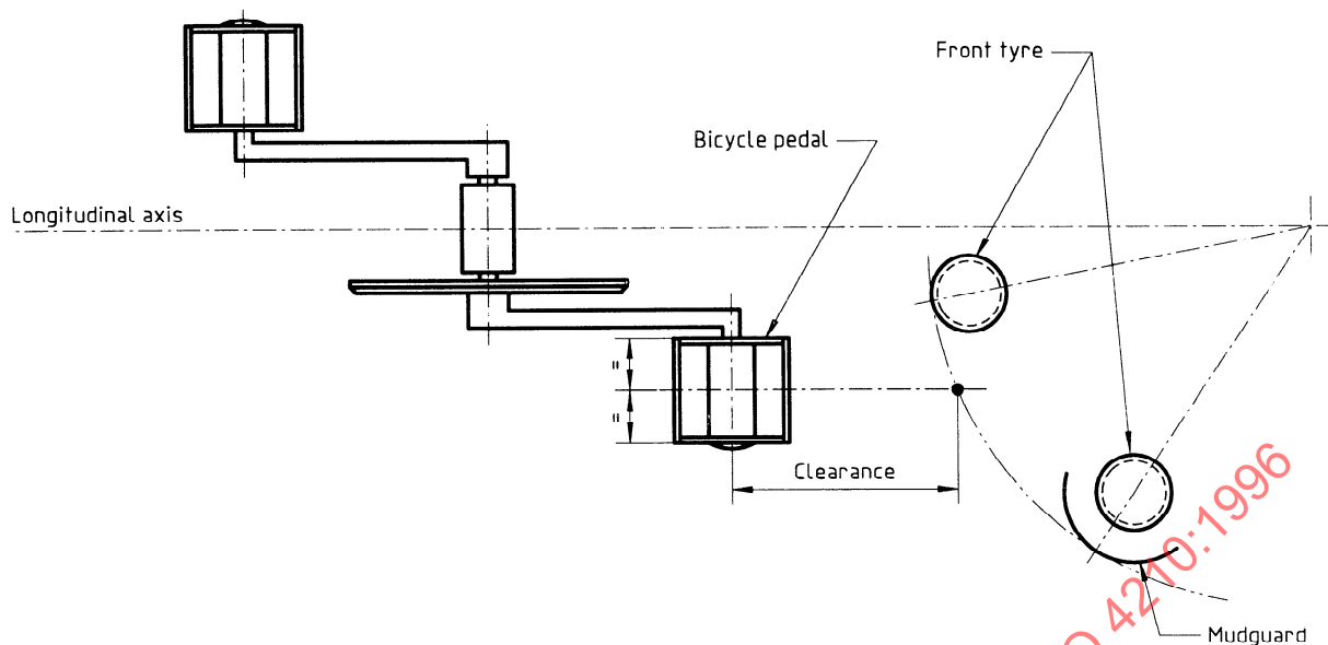
Figure 4 — Toe clearance
