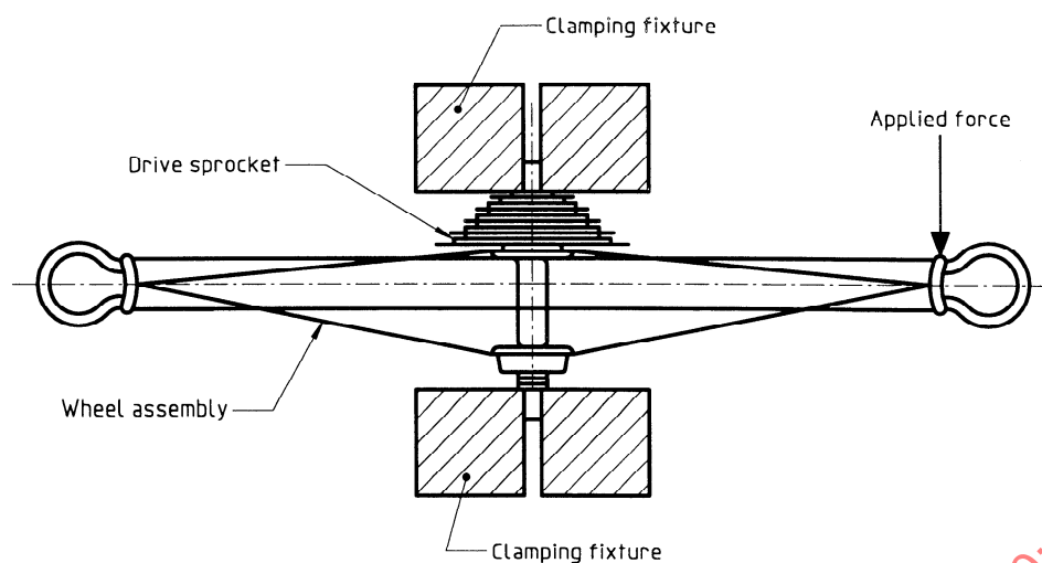
Figure 26 — Static load test on wheel
