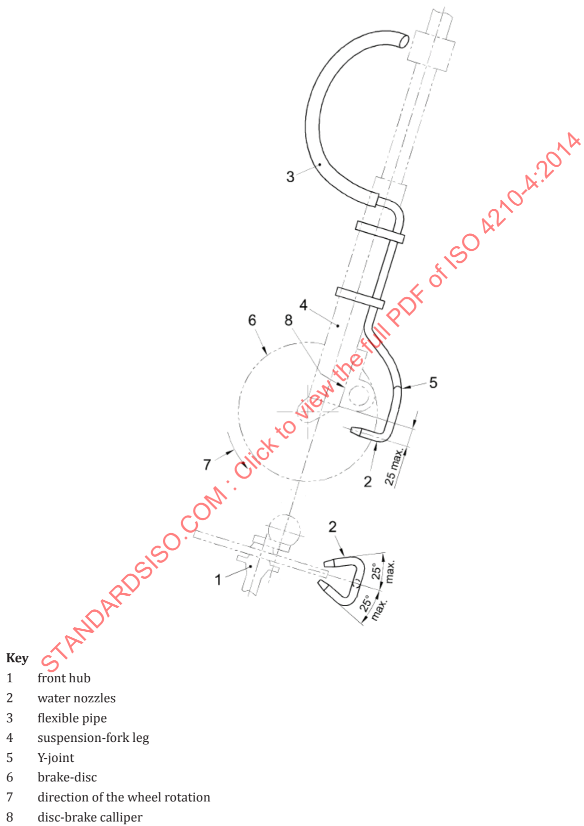
Figure 11 — Water nozzles for disc-brake (front)
