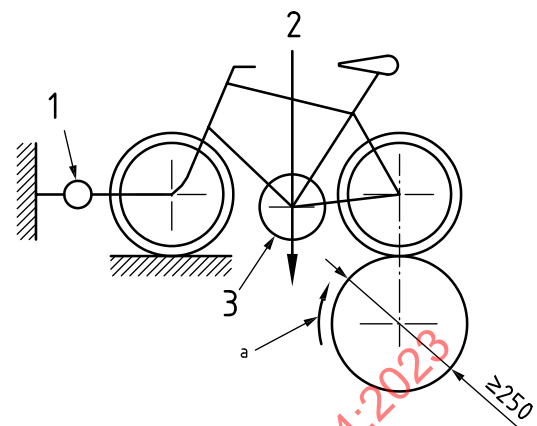
b) Testing the rear brake
