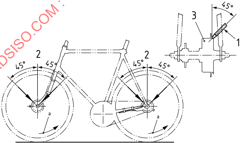
Figure 8 — Water nozzles for rim-brake (rear)
