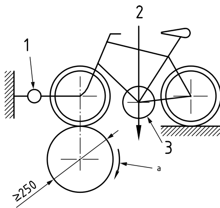
a) Testing the front brake
