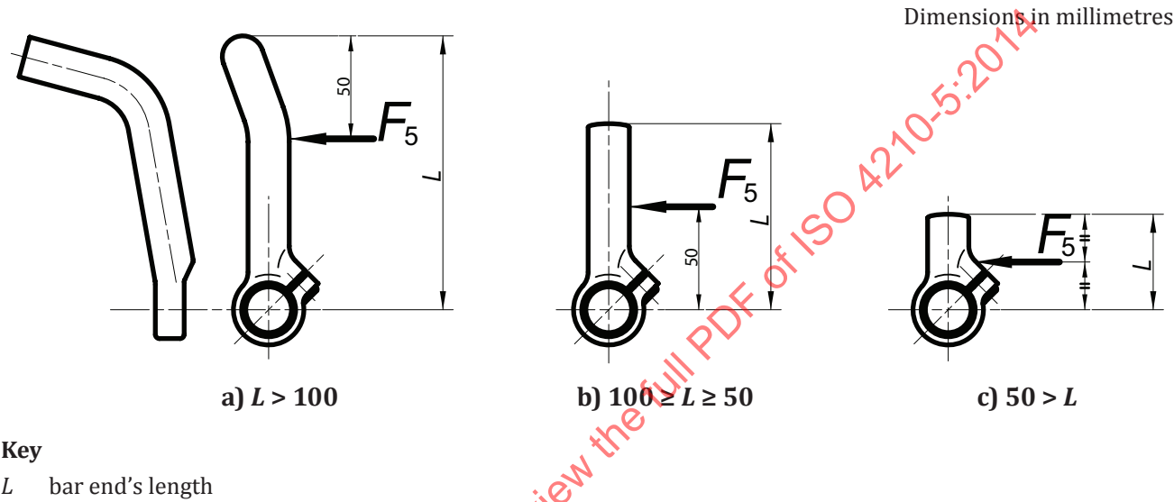
Figure 8 — Bar end to handlebar — Torsional security test
