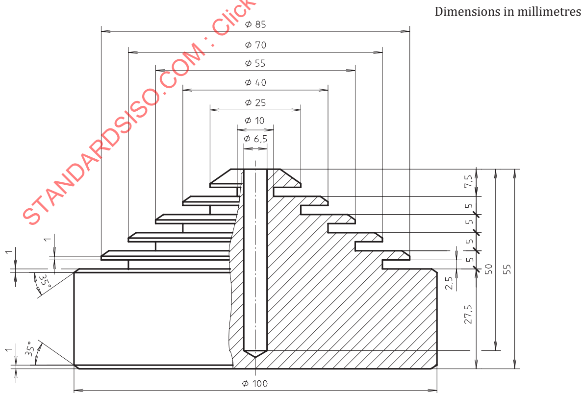
Figure 1 — Aluminium block used as heat source
