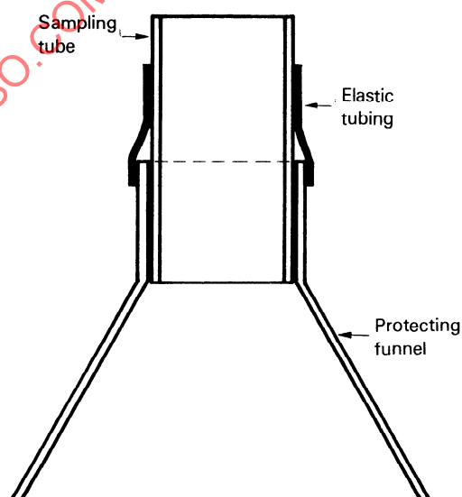
Figure 2 — Air intake with protecting funnel
