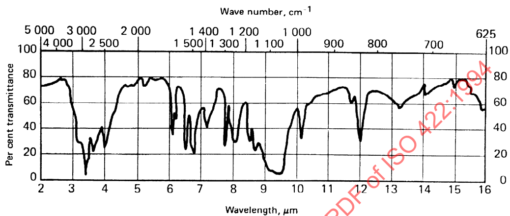
Figure 1 — Reference infrared spectrum of p -methylaminophenol sulfate (KBr plate)
