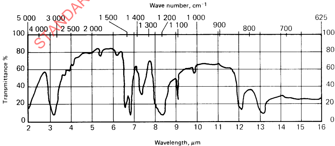
FIGURE — Reference infra-red spectrum of hydroquinone (KBr plate)
