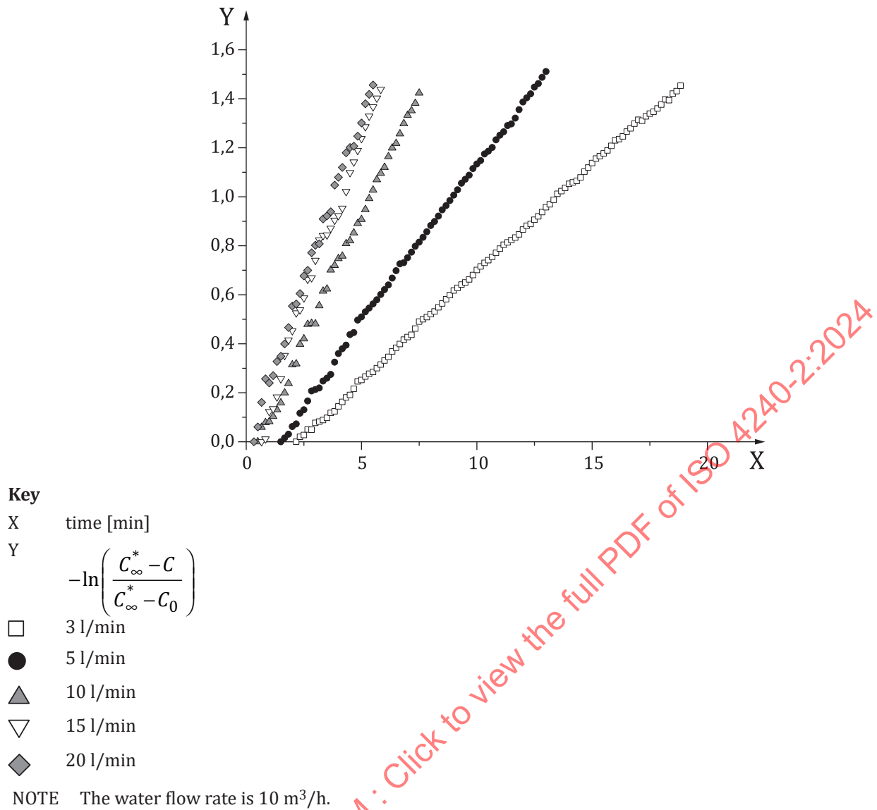
Figure A.3 — Data analysis of DO for K_{L,a} calculation
