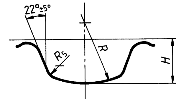
Figure 3 — Well contour — Option 1
