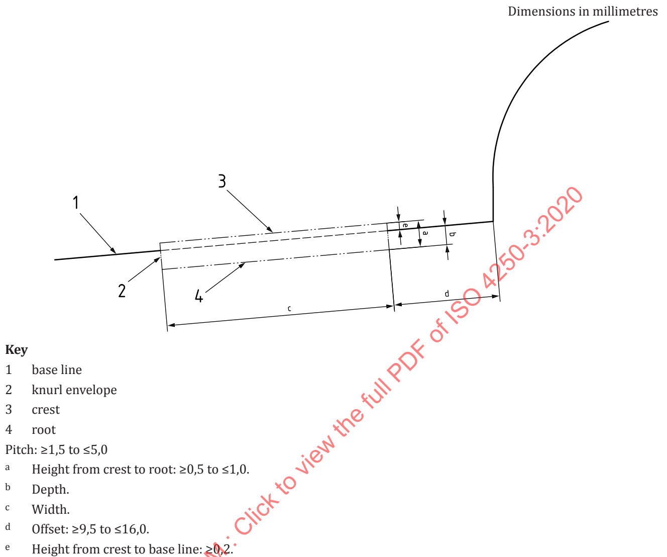
Figure 7 — Knurling detail
