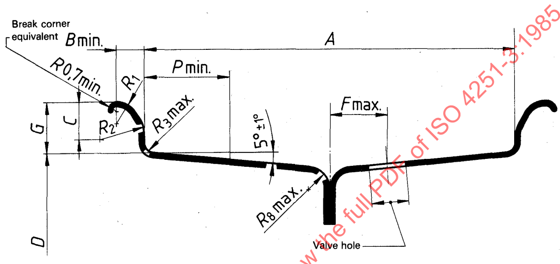
Figure 7 — Contour of divided rims
