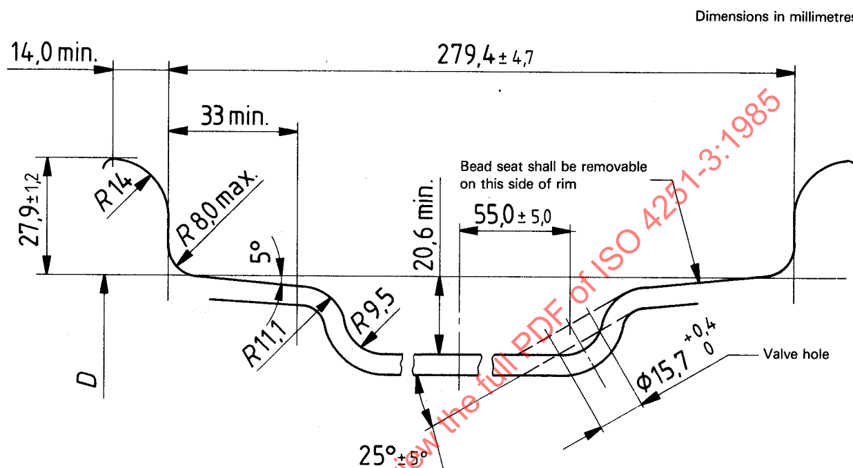
Figure 4 — Contour of semi-drop centre rim 16.1 — 11 SDC
