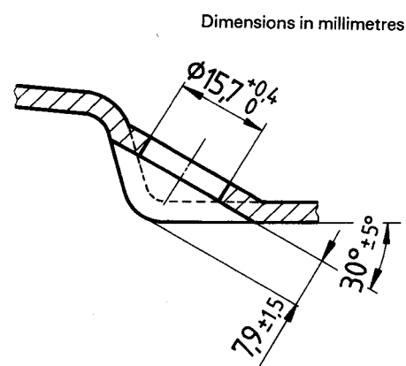
Figure 6 — Location of valve hole in corner of well
