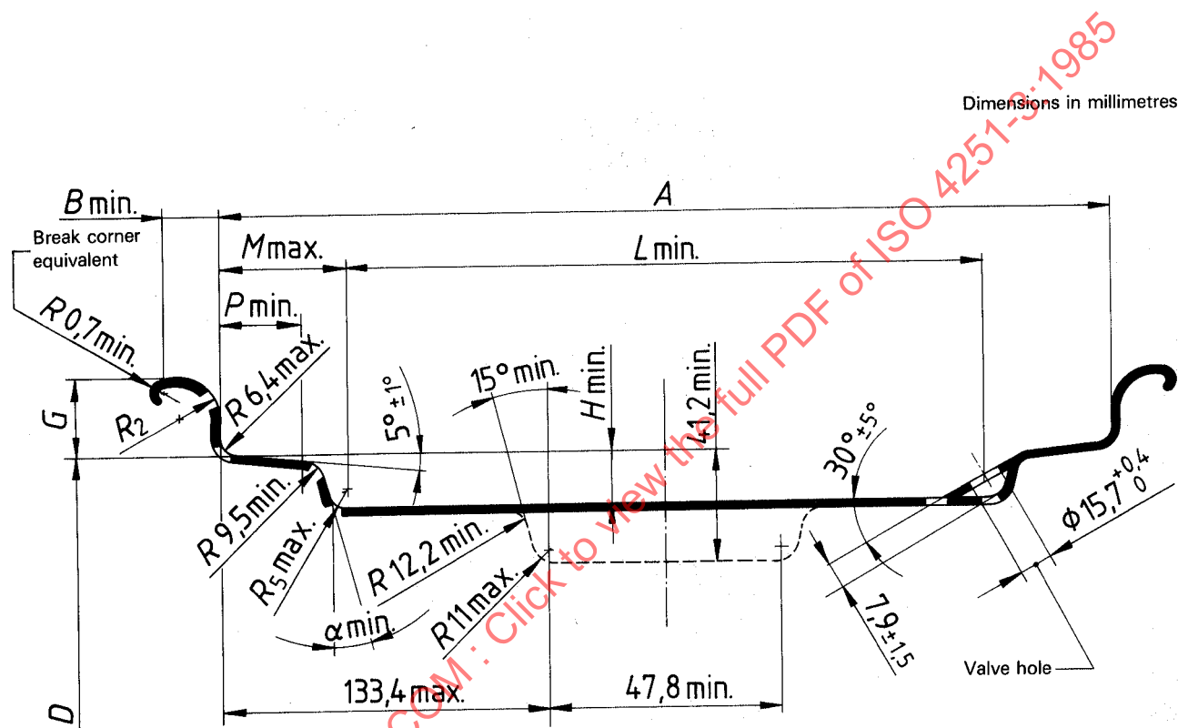
Figure 2 — Contour of W and DW rims
