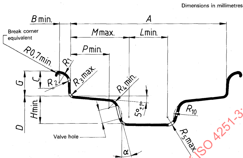
Figure 3 — Contour of other drop centre rims
