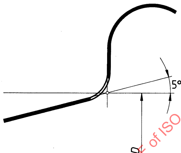
Figure 1 — Rim flange
