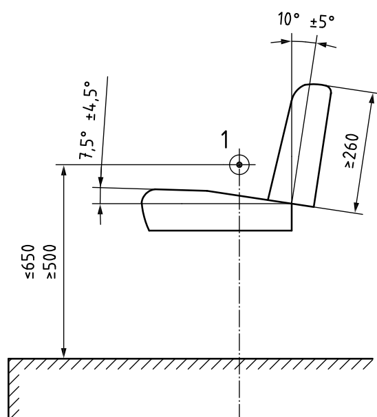
a) Intermediate seat adjustment
