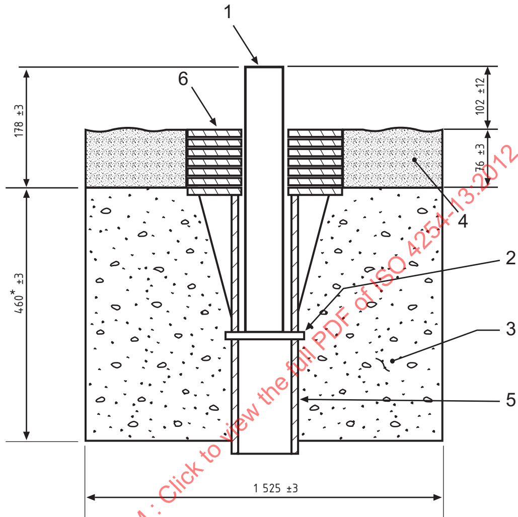
a) Example of a cutting-element impact test fixture configuration surrounded by sand
