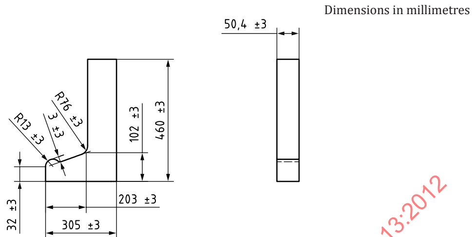
Figure 3 — Foot-probe test equipment
