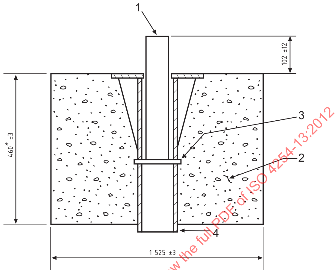
b) Example of a cutting-element impact test fixture configuration in concrete
