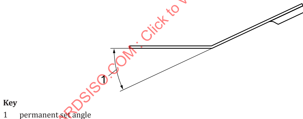
Figure 1 — Permanent set angle of cutting element after the bend test
