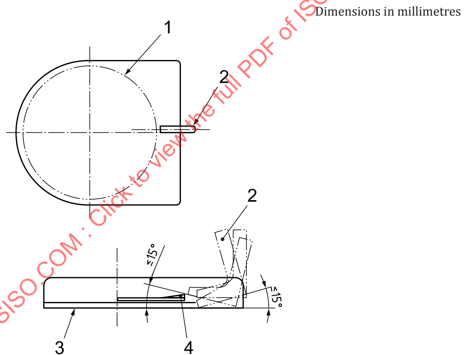
Figure 3 — Foot-probe test equipment
